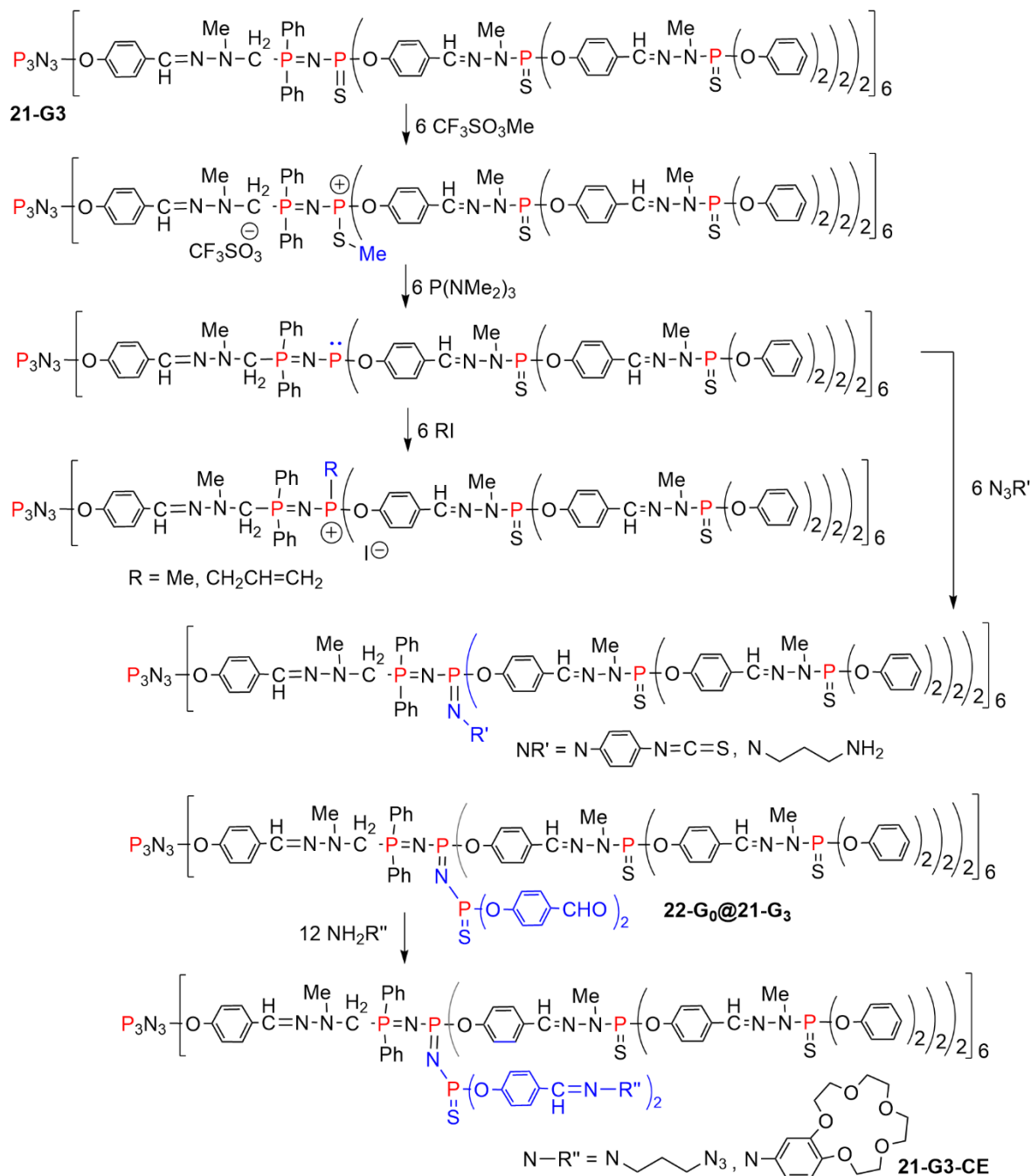
Scheme 21. Different types of reactions carried out on the P=N-P=S linkages in the internal structure of dendrimer 21-G3 .
