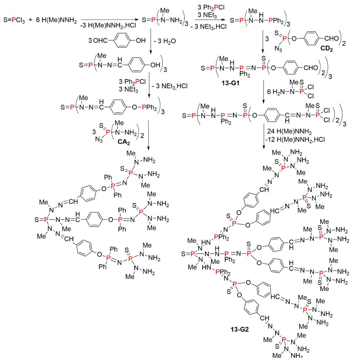
Scheme 13. Synthesis of small dendrimers using the Staudinger process.
