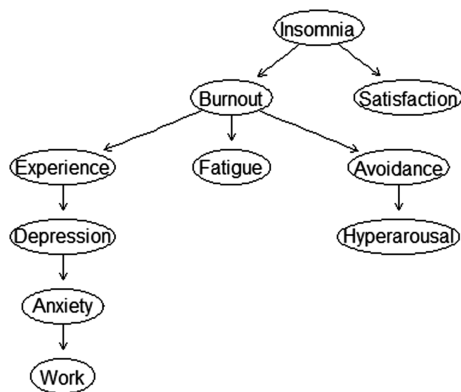
FIGURE 3 The DAG illustrates the years of nursing experience, mental health variables and work impairment network. The DAG represents the cause-and-effect relationships between the variables
