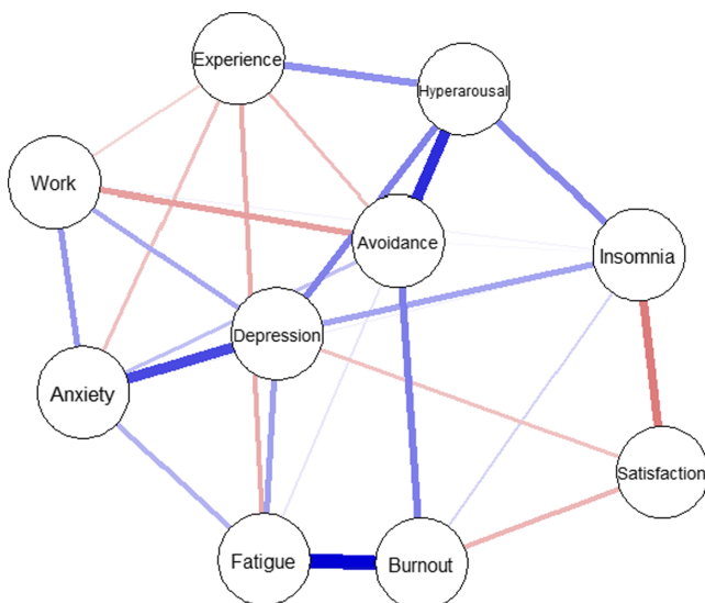
FIGURE 1 The LASSO graph illustrates the regularized partial correlation among years of experiences, mental health variables and work impairment. Positive correlations are shown with blue-coloured edges, while red-coloured edges are used for indicating negative correlations
