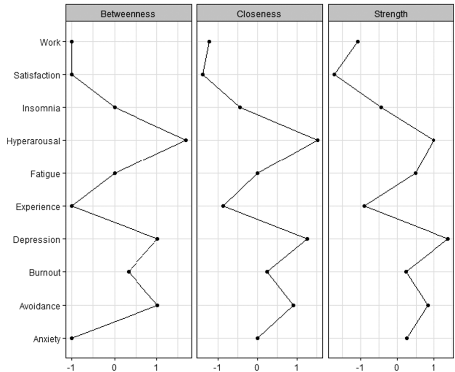
FIGURE 2 The z-scored centrality indices, betweenness, closeness and strength in the network. A z-score higher than zero shows a higher centrality in the network
