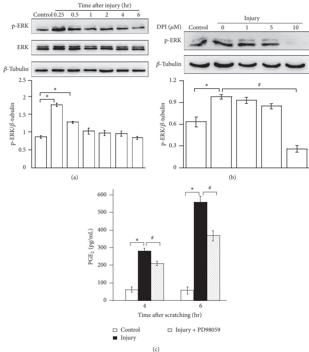
FIGURE 3: Participation of ERK activation in scratching injury-induced release of ROS and PGE 2 . (a) The change of p-ERK and ERK in HaCat cells treated with scratching injury for different periods of time as indicated. The protein levels of p-ERK and ERK were determined by immunoblot analysis and normalized to β-tubulin. (b) The level of p-ERK was decreased in HaCat cells preincubated with different concentrations of DPI for 30 min followed by scratches for 0.5 hr. (c) The dependence of PGE 2 production caused by scratching injury on ERK activation. Values are means ± SEMs of three replicates. * and # indicate p < 0.05 compared with undamaged control cells and with scratched cells, respectively.
