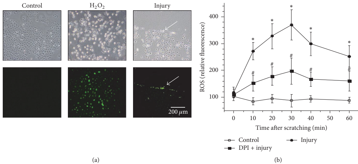
FIGURE 1: Rapid formation of ROS induced by scratching injury in HaCat cells. (a) The intracellular ROS were visualized by the reaction with probe carboxy-H 2 DCFDA under fluorescent microscopy. Cells without damage worked as negative control, while H 2 O 2 treated cells were used as positive control. (b) The quantities of ROS were shown after scratching for undamaged control cells, damaged cells, and damaged cells plus DPI treatment. Data are representative of three independent experiments with triplicate samples. * and # indicate p < 0.05 compared with undamaged control cells and with scratched cells, respectively.
