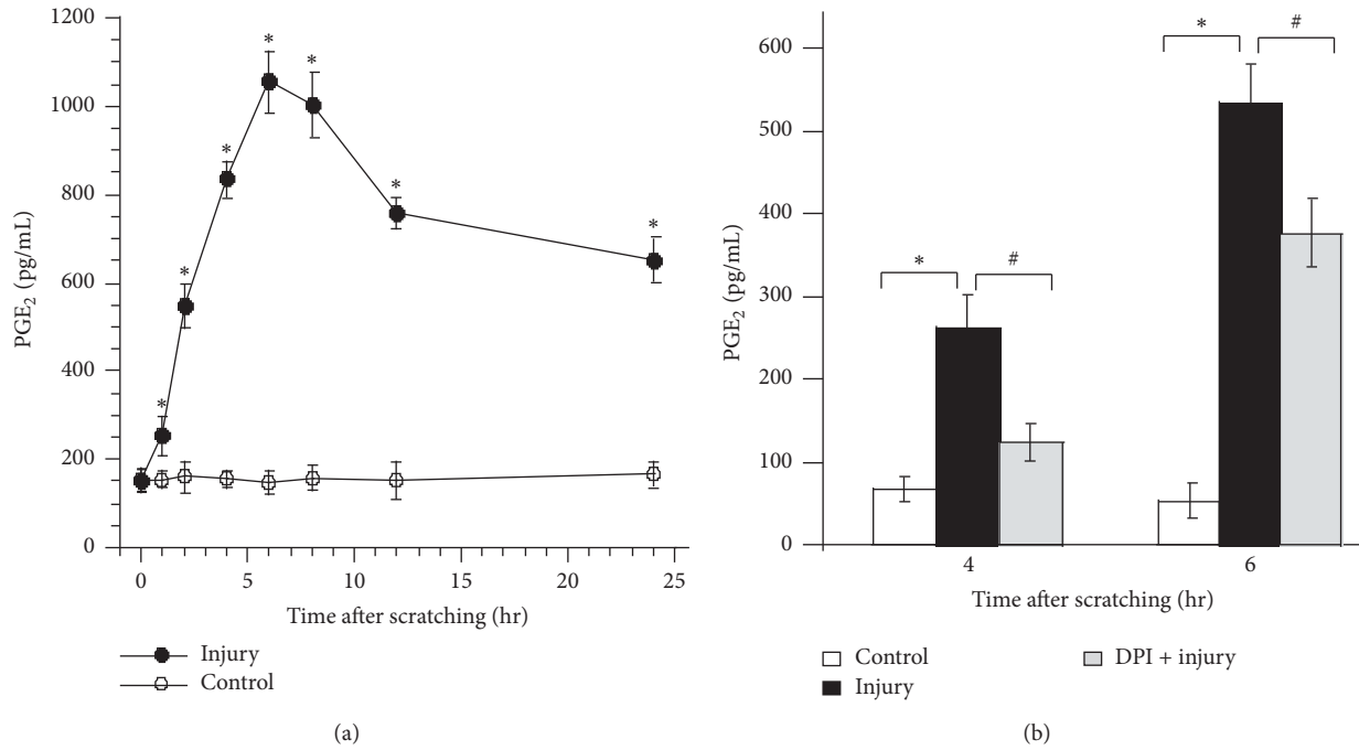
FIGURE 2: Scratching-injury-induced PGE 2 production and the dependence on ROS. (a) PGE 2 secretion by HaCat cells after scratches. PGE 2 was measured by ELISA in different periods of time as indicated. (b) Suppressed secretion PGE 2 by NOX/ROS inhibitor. Values are means \pm SEMs of three replicates. * and # indicate p < 0.05 compared with undamaged control cells and with scratched cells, respectively.
