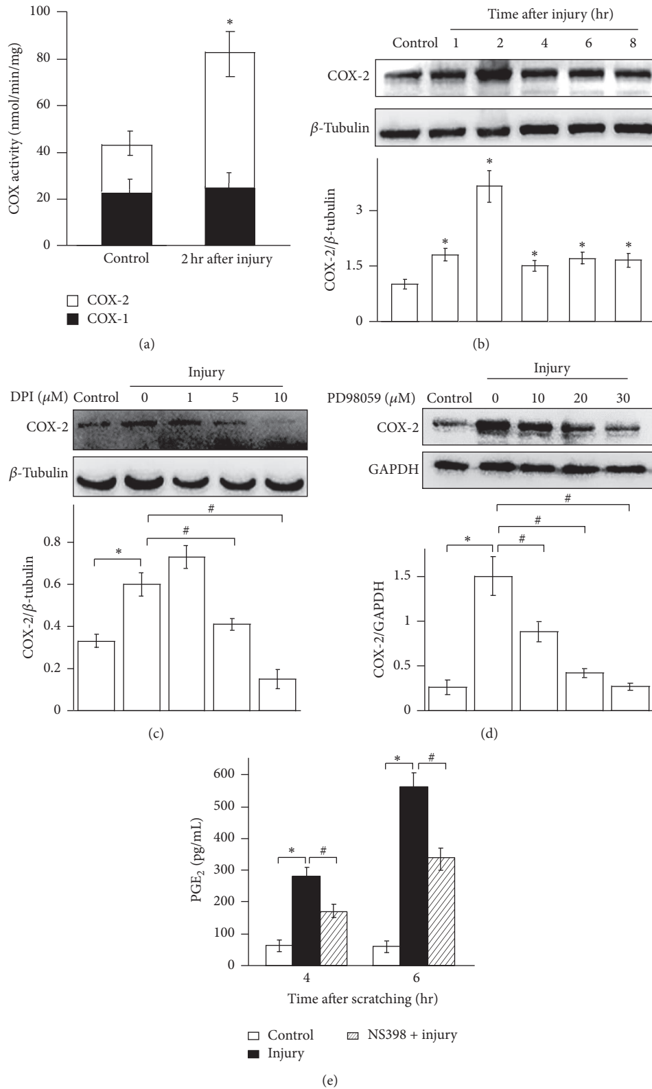
FIGURE 4: Injury-induced PGE 2 release mediated by COX-2, not COX-1. (a) COX-1 and COX-2 activity of uninjured or injured HaCat cells were measured by COX activity assay. (b) COX-2 expression was increased in HaCat cells treated with scratching injury for different periods of time as indicated. The protein levels of COX-2 were determined by immunoblot analysis and normalized to β-tubulin. (c) The induced expression of COX-2 in HaCat cells was suppressed by NOX/ROS inhibitor DPI. (d) The induced expression of COX-2 in HaCat cells was suppressed by ERK inhibitor. (e) The induced expression of COX-2 in HaCat cells was suppressed by a COX-2 inhibitor. Values are means ± SEMs of three replicates. * and # indicate p < 0.05 compared with undamaged control cells and with scratched cells, respectively.
