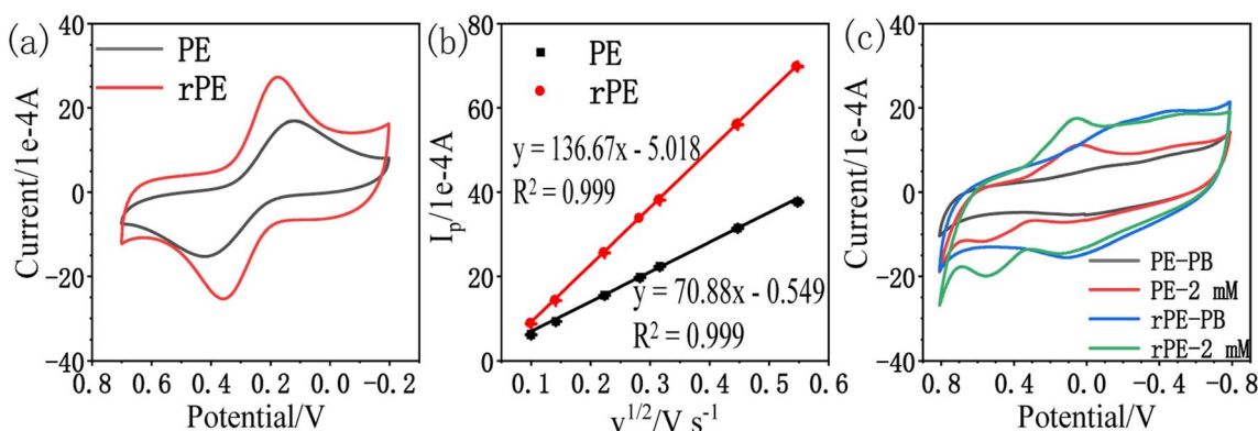
Fig. 2 (a) CVs of the paper electrodes in 1 mM \text{K}_3\text{Fe}(\text{CN})_6 in 1 M KCl. Scan rate = 50 mV s -1 . (b) Plots of oxidation peak current ( I_p/1 \times 10^{-4} A) vs. square root of the scan rate ( \nu^{1/2} ) for PE and rPE. (c) CVs of PB (pH 7) and 2 mM amitrole. Scan rate = 50 mV s -1 .
