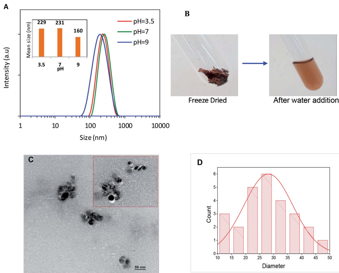
Fig. 2 (A) Particle size distribution of hybrid levans-Ag/AgCl suspension at different pH, measured by DLS, and (B) freeze-dried levans-Ag/AgCl after addition of water; (C) TEM image of hybrid levans-Ag/AgCl NPs obtained under 0.5% (w/w) levans solution containing AgNO 3 ( 5 \times 10^{-3} M) exposed to UV-light during 30 min; (D) size distribution histogram of the nanoparticles measured from the TEM images.
