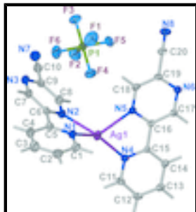
Fig. 1. The atom-numbering scheme of the title compound with displacement ellipsoids drawn at the 30% probability level.
