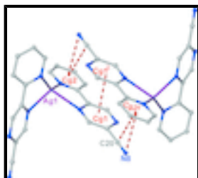
Fig. 2. The C\equiv N \cdots \pi (pyridyl) and \pi - \pi interactions between the mononuclear units, forming the dimer in the title complex.
