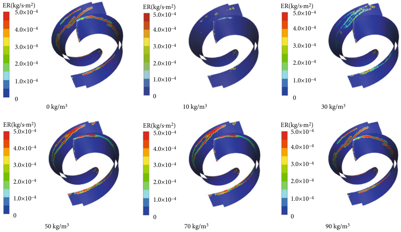
(a) Smooth vane
