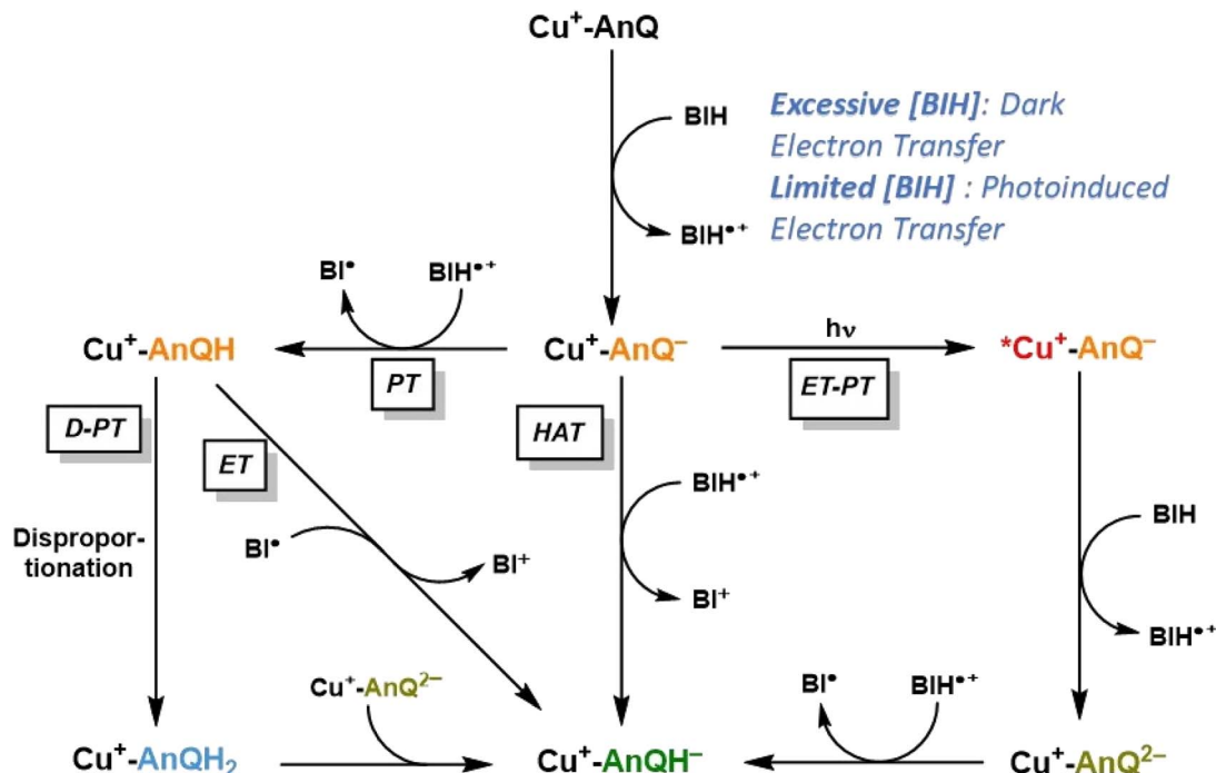
Scheme 4 Proposed reaction mechanism of charge accumulation of Cu + -AnQ with BIH. PT = proton transfer; ET = electron transfer; D = disproportionation; HAT = hydrogen atom transfer.
