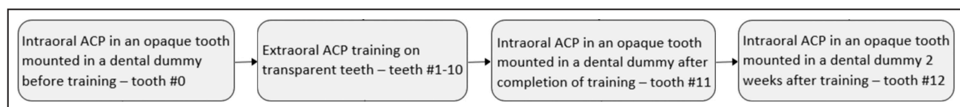
Figure 4. Training workflow
