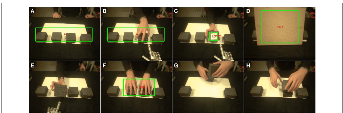
FIGURE 4 | Scenes perceived through the eyes of the iCub robot during Experiment 3. Labeled green rectangles indicate visual features recognized by the robot. The robot chose (by pointing to) one of four cubes on a table ( A,B ). The human revealed the hidden side of the indicated cube. One of the cubes had a circle on its hidden face, indicating a reward ( C ). At the end of a
