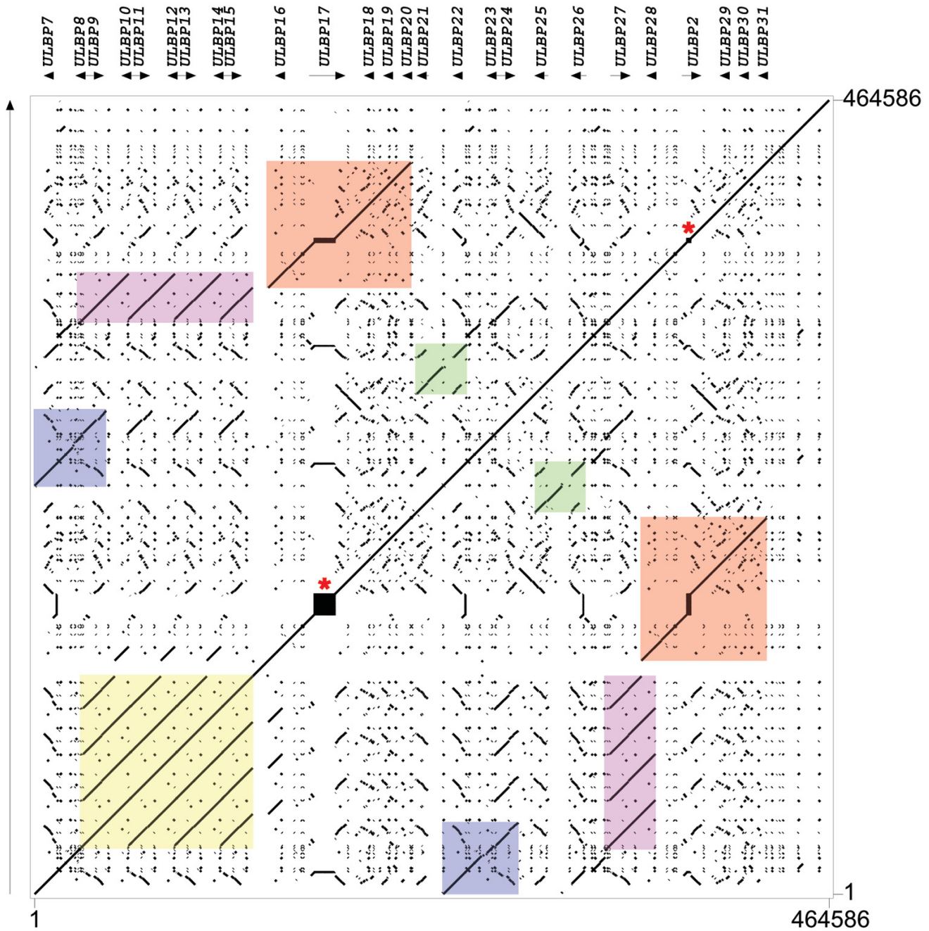
Figure 3 Internal sequence identity plot of the major ULBP cluster. Sequence numbers displayed on the X- and Y-axes indicate alignment orientation, originating in the lower left corner. The center line represents identity; other lines indicate regions of internal sequence identity. Genes are annotated above the figure with arrows indicating orientation. Nucleotide sequences used to construct the major ULBP cluster are listed in Table 1. The duplication of ULBP28-ULBP31 to form ULBP16-ULBP20 is within the red shaded area. The cattle specific repeat regions within ULBP17 and ULBP2 are indicated by red asterisks. The duplication of ULBP7-ULBP9 corresponding to ULBP22-ULBP24 is within the blue shaded area. The duplication of ULBP21-ULBP22 corresponding to ULBP25-ULBP26 is within the green shaded area. The tandem duplications of ULBP9 and ULBP10, ULBP11 and ULBP12, ULBP13 and ULBP14, and ULBP15 and ULBP16 are within the yellow shaded area, and lines showing their similarity to the ULBP27 region are within the violet shaded area.
