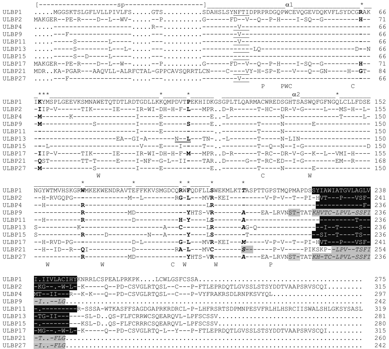
Figure 4 Protein alignment of the cattle ULBP family. Alignment gaps are represented by periods, and aligned ULBP sites sharing identity with cattle ULBP1 are represented by dashes. The signal peptide region (sp) is represented by dashes within brackets above the alignment. The \alpha 1 and \alpha 2 domains are designated by an underscore above the alignment. Universally conserved cysteine, proline, and tryptophan residues are annotated with Cs, Ps and Ws, respectively, beneath the alignment. Predicted N-glycosylation motifs are represented by underlined text in the alignment. Transmembrane domains are represented by black shaded background. Predicted GPI anchor motifs are represented by gray shaded background, and the associated downstream hydrophobic regions are indicated by italicized text with gray shaded background. Positively selected sites are indicated by asterisks above the alignment, and posterior probabilities associated with each positively selected site (see Table 2.5) are represented within the alignment by normal text (probability > 0.90), bold text (probability > 0.95), and italicized bold text (probability > 0.99).
