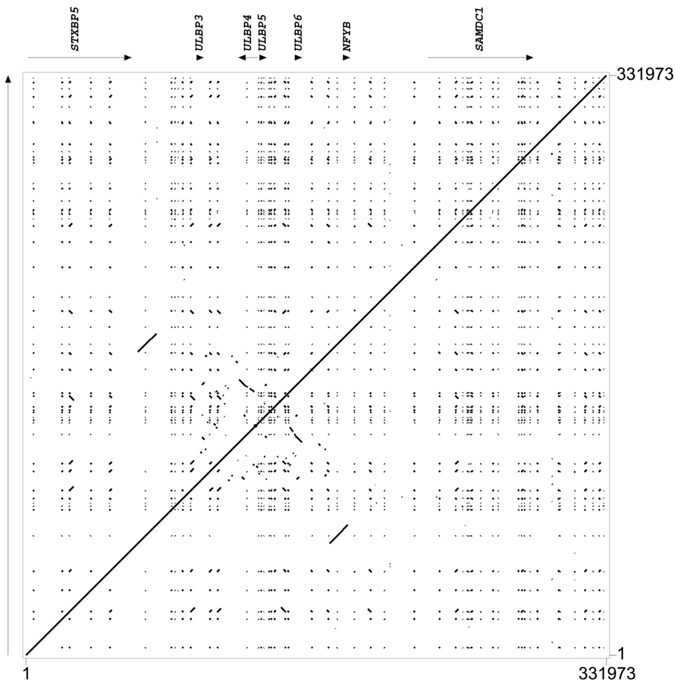
Figure 2 Internal sequence identity plot of the minor ULBP cluster. Sequence numbers displayed on the X- and Y-axes indicate alignment orientation, originating in the lower left corner. The central diagonal line represents identity; other lines indicate regions of internal sequence identity. Genes are annotated above the figure with arrows indicating orientation. Nucleotide sequences used to construct the minor ULBP cluster are listed in Table 1.
