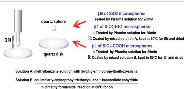
Fig. 2 The schematic representation for measuring the frictional properties of different microspheres.
