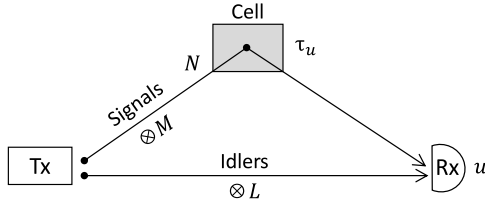
Fig. 1. Quantum reading of a memory cell. A memory cell encodes a bit u in a lossy channel with transmissivity \tau_u . The cell is read by a transmitter (Tx), which irradiates M signal modes and N mean total photons over the cell, plus extra L idler modes sent to the output. The receiver (Rx) performs a generally joint measurement of signals and idlers, decoding the bit u up to some error probability p_{\text{err}} . Quantum reading corresponds to using a quantum source of light for the Tx so that we outperform any classical source in the readout of the bit. The scheme can be realized in reflection or in transmission, as done in our experiment.
