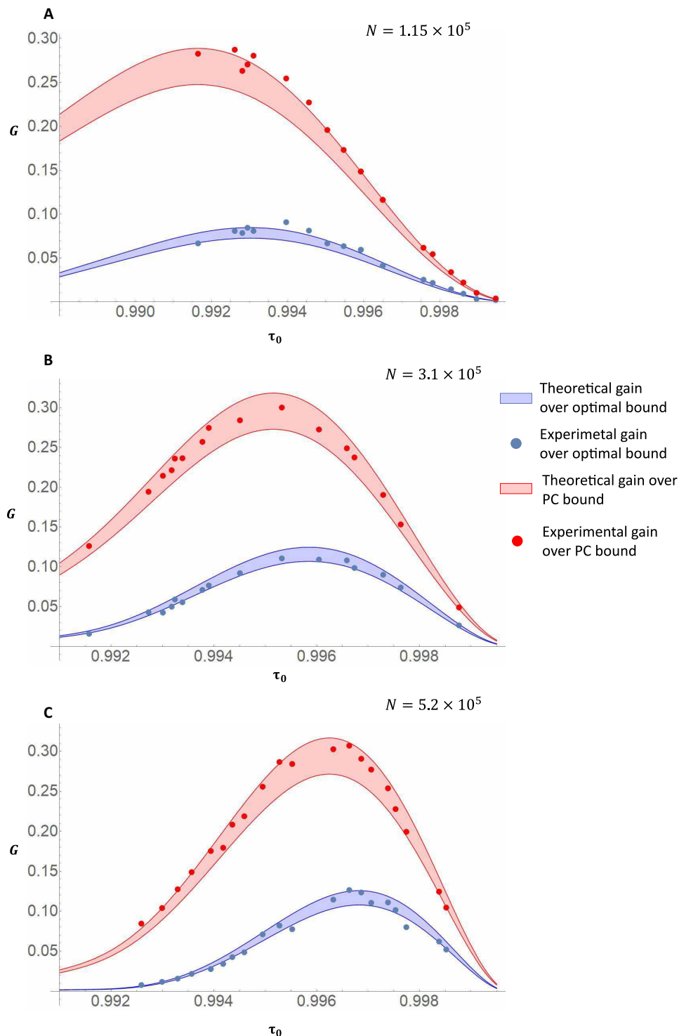
Fig. 4. Experimental gain G of quantum reading (bits) as a function of the lower transmissivity \tau_0 . The three panels refer to different mean photon number in the signal beam: (A) N = 1.15 \cdot 10^5 , (B) 3.1 \cdot 10^5 , and (C) 5.2 \cdot 10^5 . Blue data refer to the gain with respect to the classical optimal bound in Eq. 1. Red data refer to the gain with respect to the classical photon-counting bound given in Eq. 6 obtained from the marginal distribution of the signal. The experimental parameters, estimated independently in a calibration step, are the mean signal energy N , the detection efficiency of signal and idler channel \eta_S and \eta_I , and the electronic noise v_e . Apart for the value of N , which is intentionally different in the three panels, the other parameters are kept fixed to: \eta_S = 0.78 and \eta_I = 0.77 v_e \sim 10^4 .
