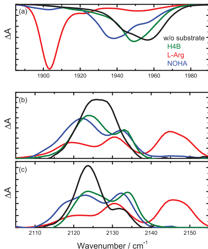
Figure 2. 4-K photolysis difference spectra of \text{iNOS}_{\text{oxy}}\text{-CO} . (a) Absorption of the heme-bound CO. (b) Photoproduct bands obtained after 10-s illumination at 4 K. (c) Photoproduct bands obtained after constant illumination during slow cooling from 160 to 4 K.
