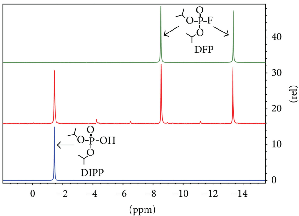
Figure 6. ^{31}\text{P} NMR spectra of pure DFP (top), partially degraded commercial DFP (middle), and a pure DIPP standard (bottom).
