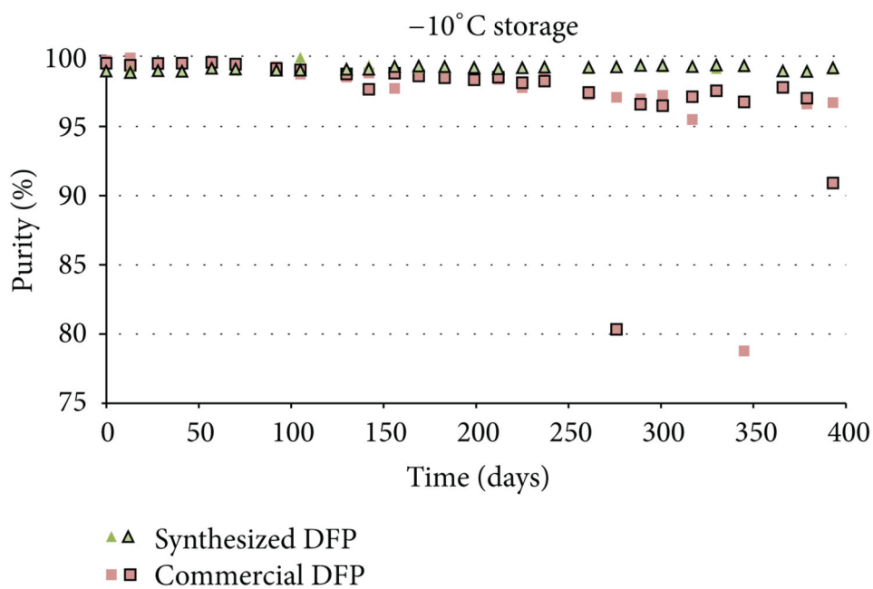
Figure 4. Purity results for synthesized DFP and commercial DFP when stored at -10^{\circ}\text{C} .
