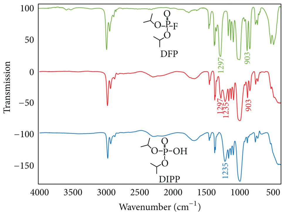
Figure 7. FT-IR spectra of pure DFP (top), partially degraded commercial DFP (middle), and a pure DIPP standard (bottom).
