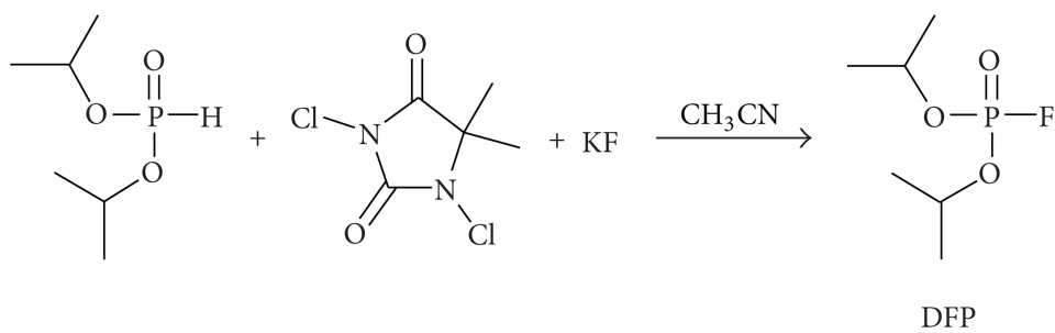
Figure 2. One-pot synthesis of DFP.
