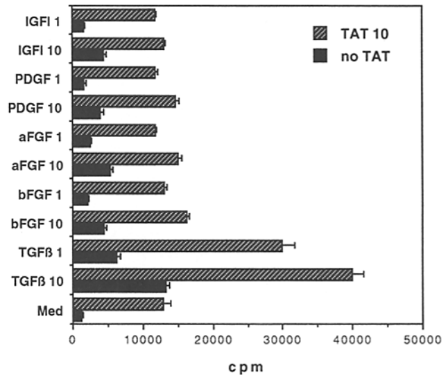
Figure 2. Tat synergy with TGFβ and other chondrocyte growth factors. Tat (10 μg/ml) and the different growth factors (concentrations shown as ng/ml) were added at initiation of culture and proliferation was measured after 96 h. Results represent mean cpm ± SEM of three experiments performed in triplicate.
