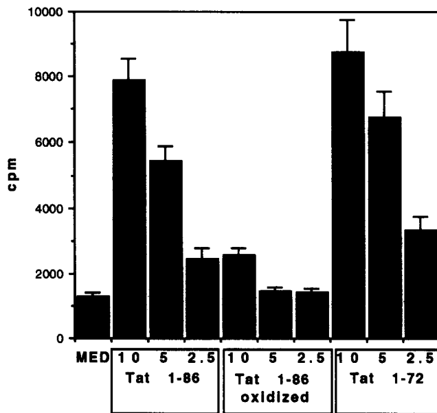
Figure 1. HIV Tat stimulates chondrocyte proliferation. Chondrocytes were stimulated with the indicated concentrations of TGFβ (ng/ml) or Tat (μg/ml) and proliferation was measured as [ 3 H]thymidine incorporation after 96 h. A shows HIV Tat dose response and comparison to TGFβ. Results represent mean cpm ± SEM of six experiments performed in triplicate. B shows specificity of HIV Tat effects. Chondrocytes were stimulated with Tat 1-86 or Tat 1-72. An aliquot of Tat 1-86 in solution was oxidized and then added to the chondrocyte cultures.
