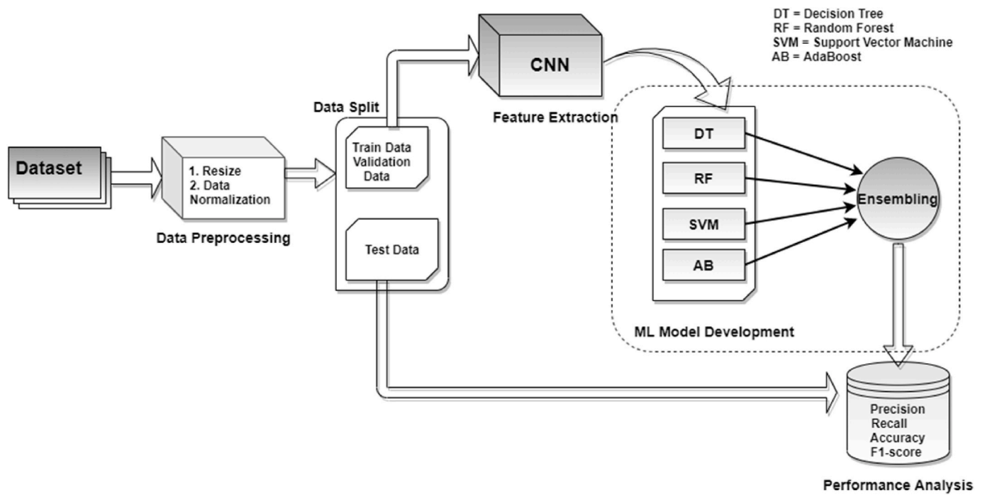
Fig. 1. Architecture of EMCNet.
