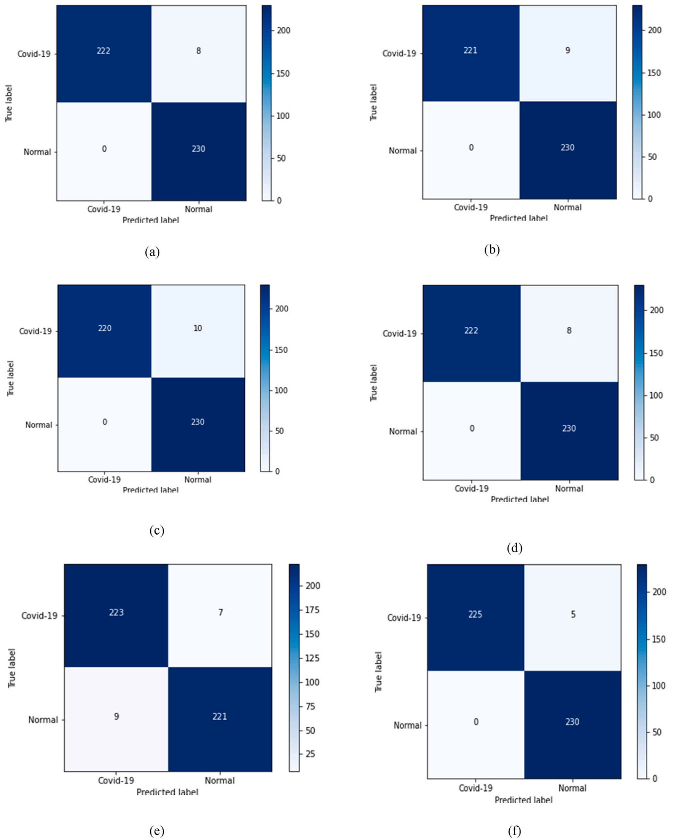
Fig. 6. Confusion matrix representation for the classifiers used in EMCNet (a) CNN (b) RF (c) DT (d) AB (e) SVM (f) Ensemble of Classifiers.
