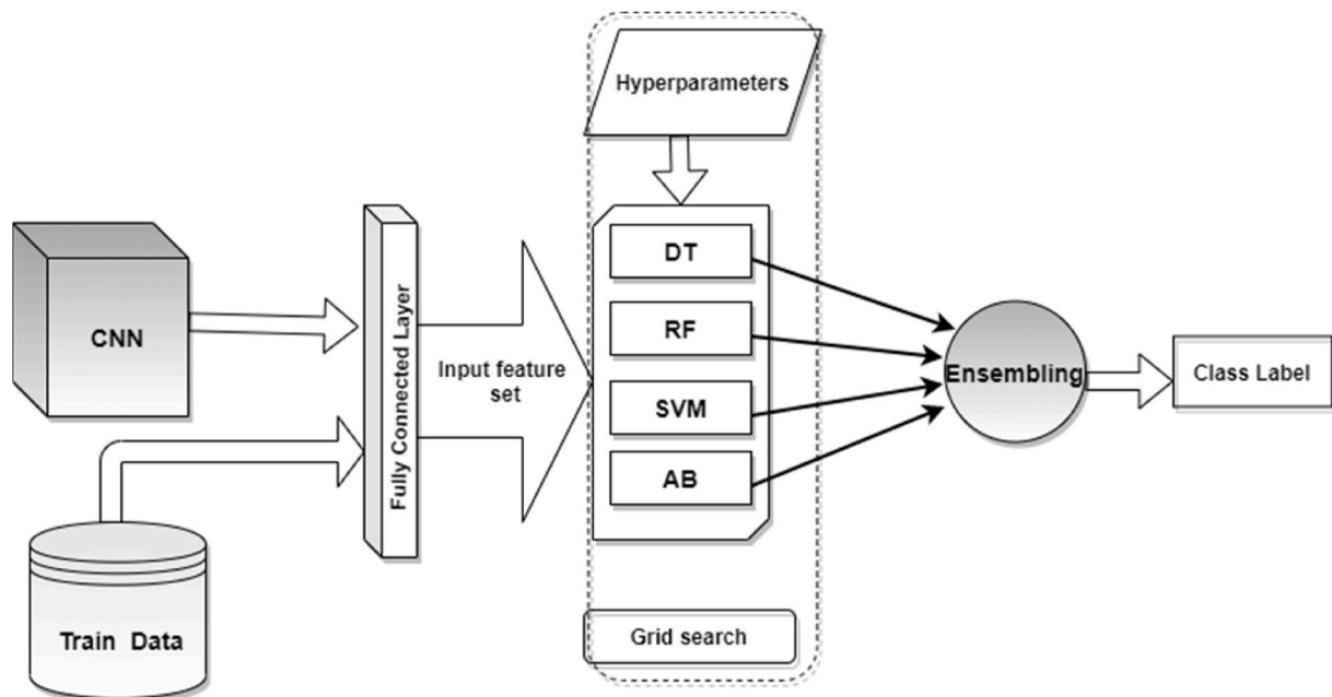
Fig. 4. Training process of ML classifiers and ensemble of classifiers.
