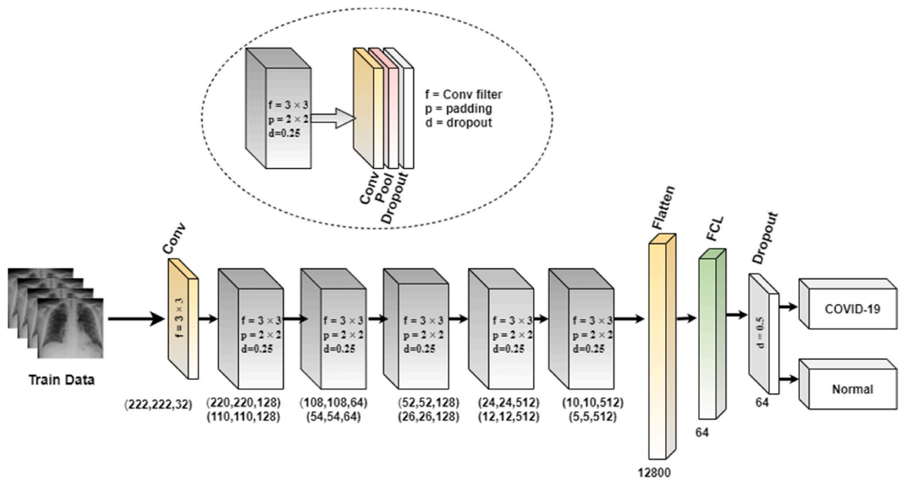
Fig. 3. Proposed CNN architecture.
