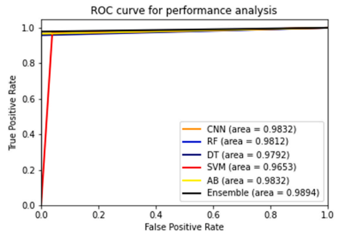
Fig. 8. ROC curve for the classifiers of EMCNet.
