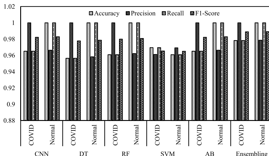
Fig. 7. Graphical representation of the performance of the models used in EMCNet for each class label.
