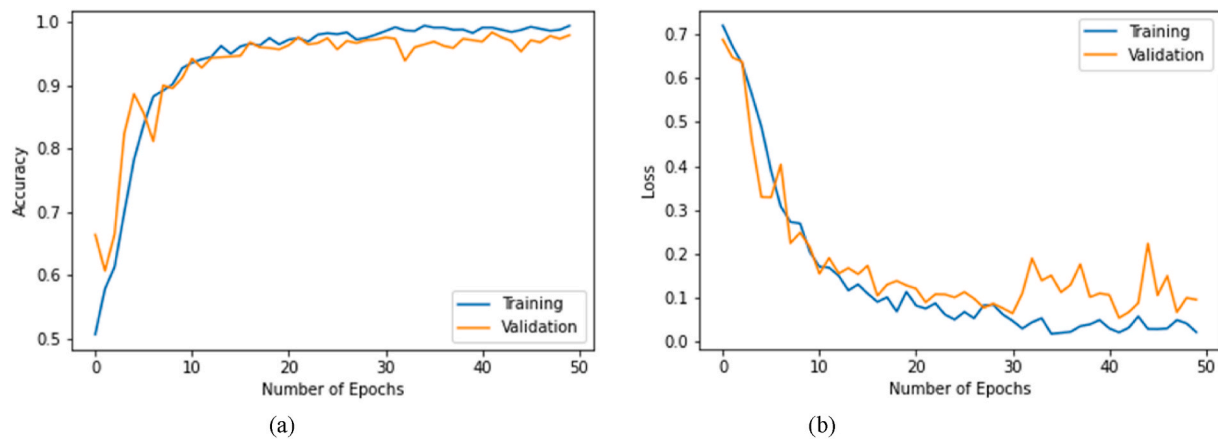
Fig. 5. Performance analysis of the CNN used in EMCNet. (a) Training and Validation Accuracy (b) Training and Validation Loss.
