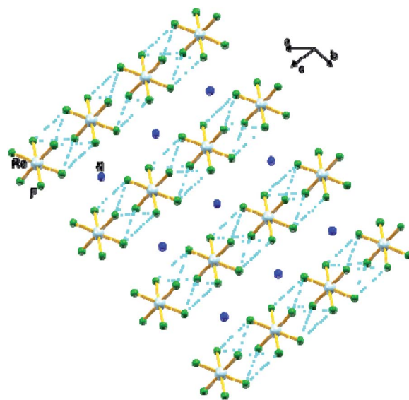
Fig. 3 View of a fragment of the crystal packing of 1 showing intermolecular \text{F}\cdots\text{F} contacts via \text{Re}\cdots\text{F}\cdots\text{F}\cdots\text{Re} (dashed aqua line). Colour of atoms: Re in light-blue, N in dark-blue and F in green.
