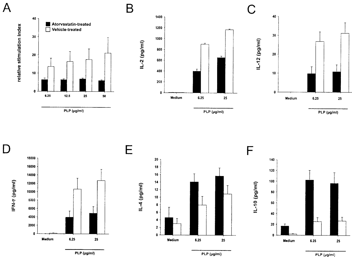
Figure 3. Atrovastatin treatment in vivo suppresses the PLP-specific priming response. Three mice per group were treated with either atorvastatin (200 \mu g per mouse) or vehicle from day 1 after immunization with PLP as described in Materials and Methods. (A) Proliferation of splenocytes in response to PLP (at the indicated concentrations) was assessed in quadruplicate cultures and expressed as stimulation index (mean \pm SEM; atorvastatin, shaded bars; vehicle, open bars). (B) Accordingly, IL-2 was determined in the supernatants. Whereas IL-12 (C) as well as IFN- \gamma (D) were found at lower concentrations in the atorvastatin-treated mice than in those vehicle-treated, levels of IL-4 (E) and IL-10 (F) were higher in supernatants from splenocytes after treatment with atorvastatin. Data are presented as mean \pm SEM; differences between atorvastatin and vehicle treatment are significant ( P < 0.05 ; Student's t test).
