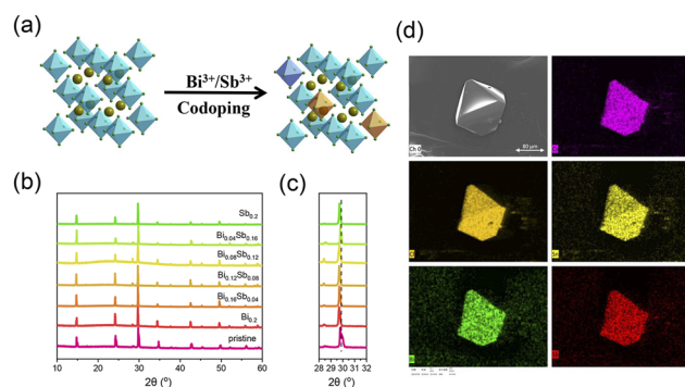
Fig. 1 (a) The diagram of \text{Bi}^{3+}/\text{Sb}^{3+} co-doping in zero-dimensional \text{Cs}_2\text{SnCl}_6 metal halides (Sn cyan, Cs dark yellow, Cl green, Bi light blue, Sb light orange). Full range (b) and selected range (c) of the PXRD pattern of measured data for \text{Cs}_2\text{SnCl}_6\text{:Bi}_{0.2-x}\text{Sb}_x ( x = 0.04, 0.08, 0.12, 0.16, 0.2 ) sample. (d) The SEM image and EDS mapping of \text{Cs}_2\text{SnCl}_6\text{:Bi}_{0.08}\text{Sb}_{0.12} .
