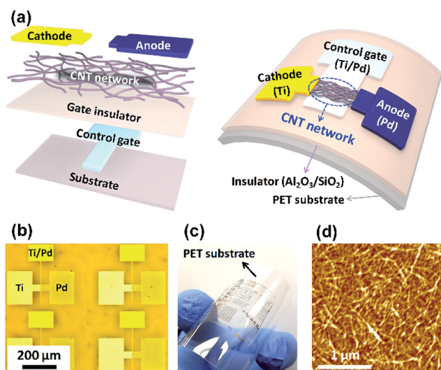
Fig. 1 (a) Schematic diagram of the flexible CNT Schottky diode with Ti as the cathode, Pd as the anode, and Ti/Pd as the embedded control gate. (b) Optical micrograph of the fabricated CNT Schottky diode on a PET substrate. (c) Optical image of the flexible CNT diode on a PET substrate. (d) AFM image ( 2.5 \times 2.5 \mu\text{m} , the z-scale is 10 nm) of the CNT network channel constructed from a 99% semiconducting CNT solution.
