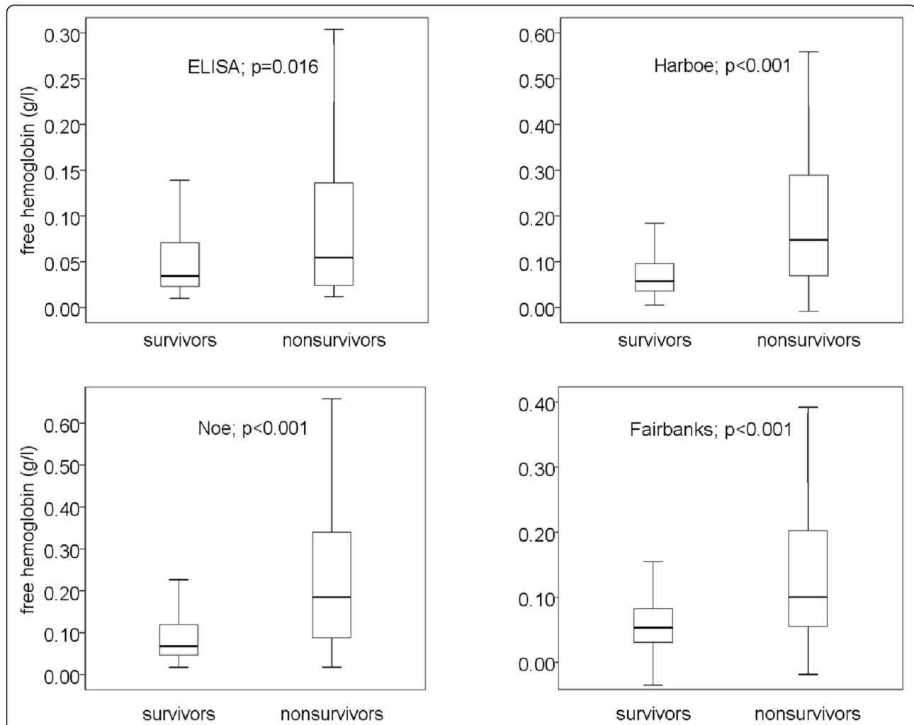
Figure 1 Free hemoglobin concentrations in survivors and non-survivors of severe sepsis as obtained by ELISA and three spectrophotometric methods. Data are given in boxplots (median, quartile, minimum, maximum). For statistical evaluation the Mann-Whitney test was used. Spectrophotometric methods were the methods of Harboe [13], Noe [14] and Fairbanks [15].
