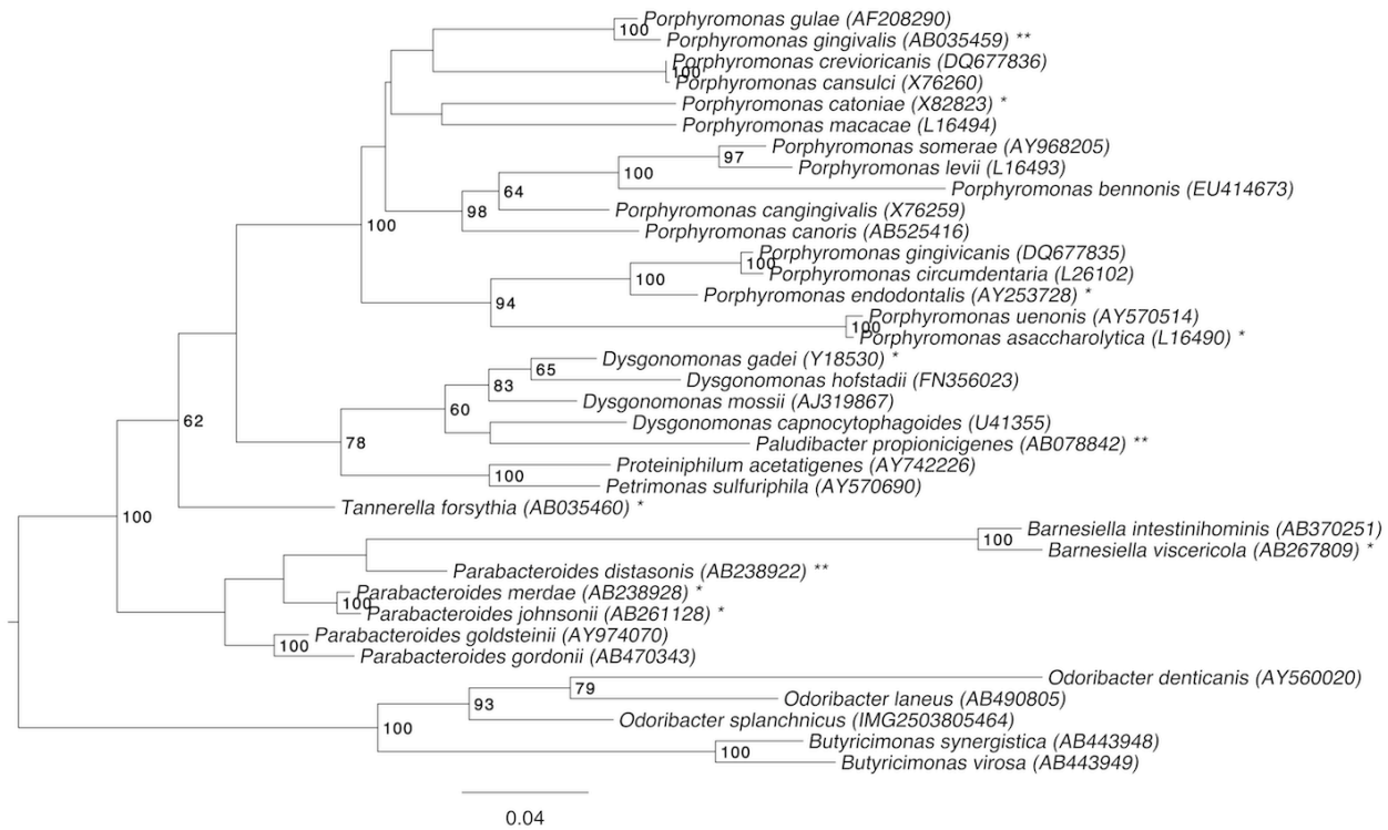
Figure 1. Phylogenetic tree highlighting the position of O. splanchnicus relative to the other type strains within the family Porphyromonadaceae . The tree was inferred from 1,401 aligned characters [11,12] of the 16S rRNA gene sequence under the maximum likelihood criterion [13]. Rooting was done initially using the midpoint method [14] and then checked for its agreement with the current classification (Table 1). The branches are scaled in terms of the expected number of substitutions per site. Numbers to the right of bifurcations are support values from 250 bootstrap replicates [15] if larger than 60%. Lineages with type strain genome sequencing projects registered in GOLD [16] are labeled by one asterisk, published genomes by two asterisks [17,18,19].
