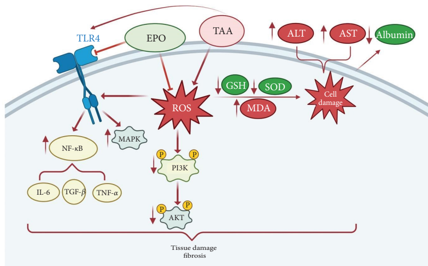
FIGURE 10: Illustration of an erythropoietin-associated pathway that suppresses the hepatic fibrosis caused by thioacetamide. EPO, erythropoietin; TAA, thioacetamide; MAPK, mitogen-activated protein kinase; ALT, alanine transaminase; AST, aspartate transaminase; GSH, reduced glutathione; MDA, malondialdehyde; SOD, superoxide dismutase; TNF- \alpha , tumor necrosis factor alpha; TGF \beta 1, transforming growth factor beta 1; IL-1 \beta , interleukin 1 beta; TLR4, Toll-like receptor 4; PI3K, phosphoinositide 3-kinase; AKT, alpha serine/threonine protein kinase 1; p, phosphorylated.
