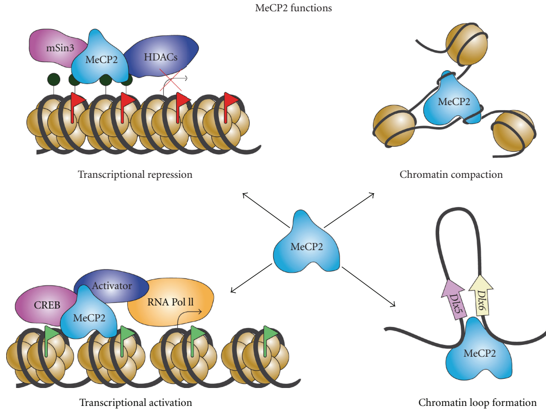
FIGURE 1: The diverse functions of MeCP2 in gene regulation and chromatin organization.
