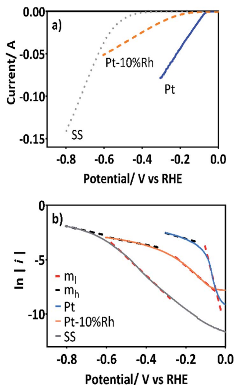
Fig. 3 (a) PC of the Pt (blue), Pt-10%Rh (orange) and SS (gray) cathodes for HER in 0.5 \text{ mol L}^{-1} \text{ H}_2\text{SO}_4 (LSV scan rate = 5 \text{ mV s}^{-1} ). (b) The corresponding Tafel plots of Pt (blue), Pt-10%Rh (orange) and SS (gray) calculated from data of plots in (a). Dashed lines show the overpotential regions at which the Tafel slopes were calculated.
