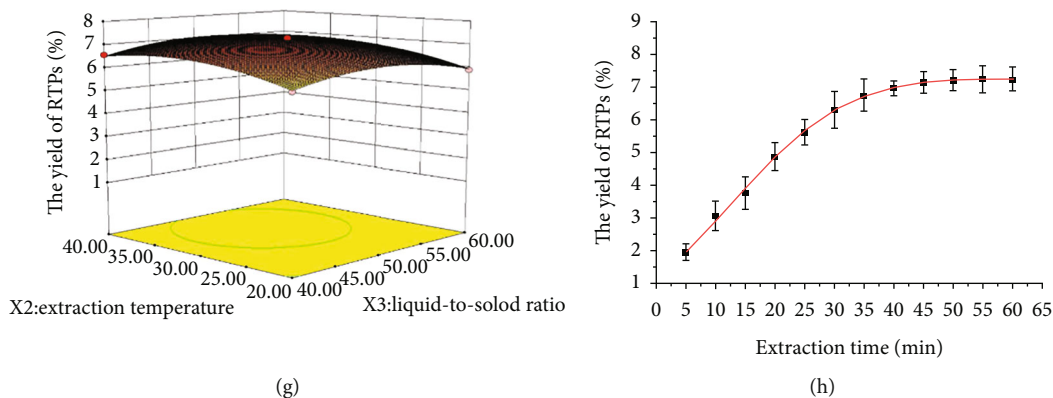
FIGURE 1: Effect on the extraction yield of RTPs. (a) A single factor for different concentrations of enzymes, (b) single factor for pH, (c) single factor for extraction temperature, and (d) single factor for liquid-to-solid ratio. (e) Response surface (3D) plot of interaction between pH ( X_1 ) and extraction temperature ( X_2 ), (f) response surface (3D) plot of interaction between pH and liquid-to-solid ratio ( X_3 ), and (g) response surface (3D) plot of interaction between extraction temperature and liquid-to-solid ratio. (h) Kinetics of UACEE process described by Weibull model. Notes: [RTPs]_{\infty} = 7.8374\% ; R^2 = 0.9936 ; k_e = 0.0521 \text{ min}^{-1} ; d = 0.9825 .
