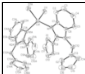
Fig. 1. View of the title complex, showing the labelled atoms and displacement ellipsoids at the 30% probability level. H atoms were omitted for clarity. [Symmetry code A: -x+1, y, -z+0.5.]
