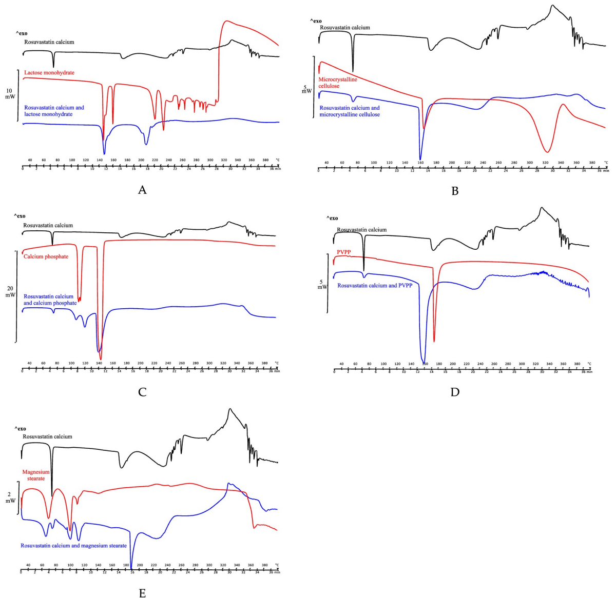
Fig 6. DSC binary (1:1) mixtures of rosuvastatin and excipients. (A) DSC of rosuvastatin, lactose monohydrate and physical mixture. (B) DSC of rosuvastatin, cellulose microcrystalline and physical mixture. (C) DSC of rosuvastatin, calcium phosphate and physical mixture. (D) DSC of rosuvastatin, PVPP and physical mixture. (E) DSC of rosuvastatin, magnesium stearate and physical mixture.
