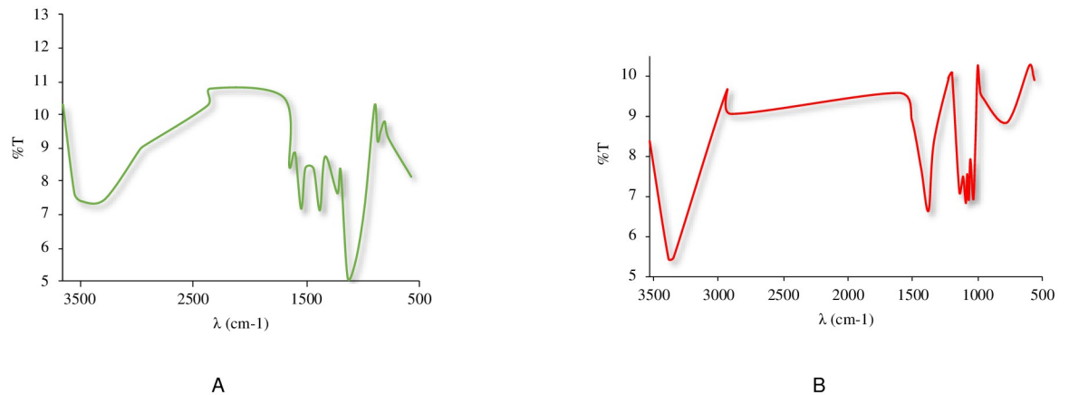
Fig 9. FT-IR binary (1:1) mixtures of rosuvastatin and excipients. (A) Physical mixture rosuvastatin and dibasic calcium phosphate. (B) Physical mixture rosuvastatin and lactose monohydrate.
