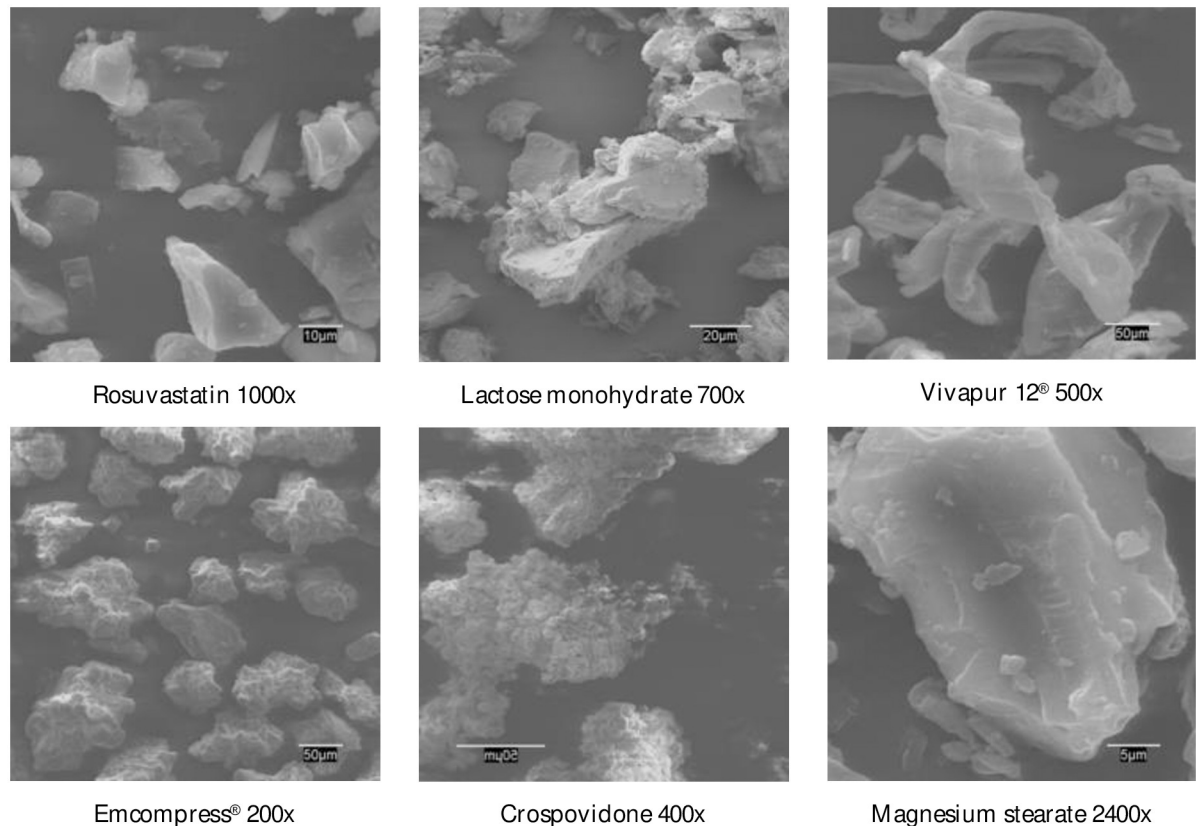
Fig 4. SEM of rosuvastatin calcium and selected excipients.
