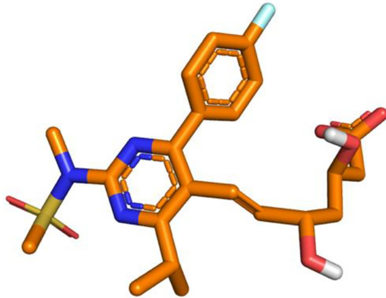
Fig 1. Rosuvastatin 3D structure. In orange are shown the carbon atoms, blue the nitrogen atoms, yellow the sulphur atom, in cyan the fluorine atom and the polar oxygen and hydrogen atoms in red and white, respectively.
