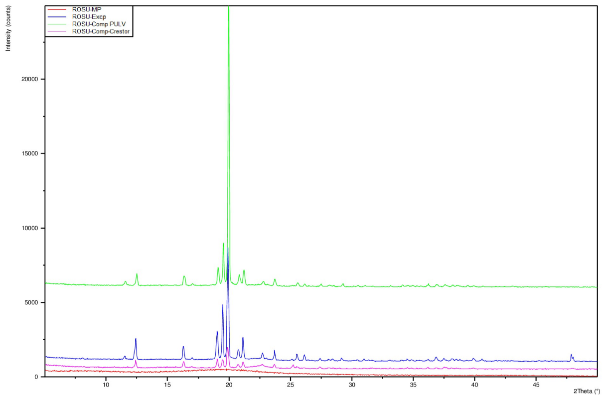
Fig 10. PXRD rosuvastatin calcium. In red is shown the PXRD of pure rosuvastatin calcium, pink the PXRD of marketed tablets, blue the PXRD of mixture drug-excipients, green the PXRD of tablets under study.
