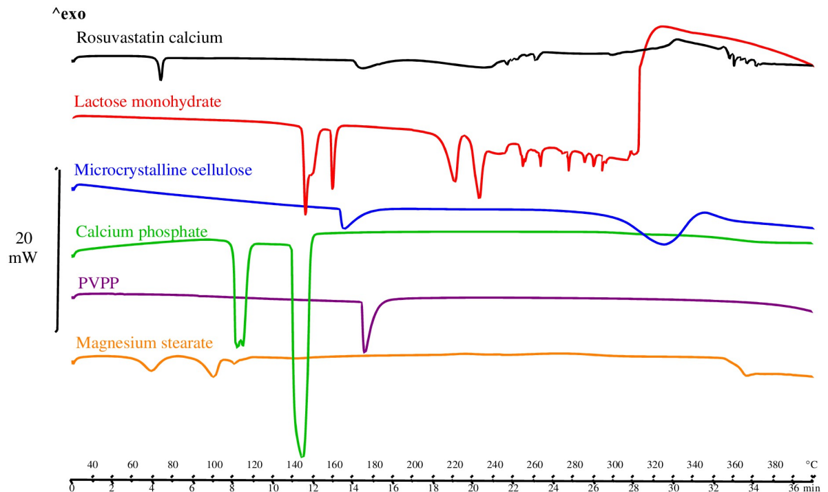
Fig 5. DSC rosuvastatin calcium and selected excipients.
