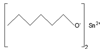
tin(II) n -hexoxide, (\text{Sn})\text{C}_6\text{H}_{13}(2)
