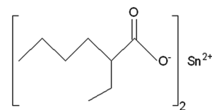
tin(II) octoate, (\text{Sn})\text{C}_8\text{H}_{15}\text{O}_2(2)
