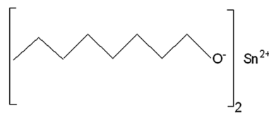
tin(II) n -octoxide, (\text{Sn})\text{C}_8\text{H}_{17}(2)
