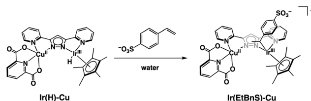
Scheme 1 Schematic representation of Ir(EtBnS)-Cu formation from the reaction between Ir(H)-Cu and StyreneS in water.
