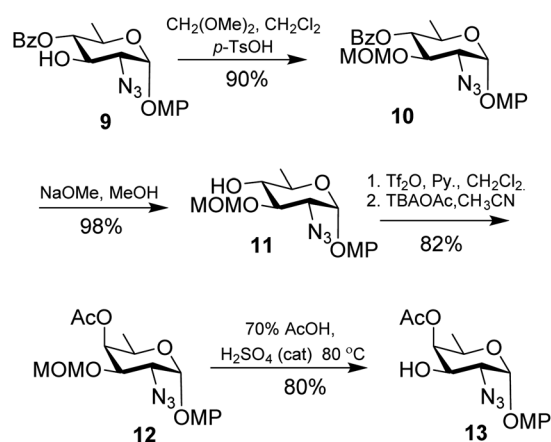
Scheme 2 Preparation of D -fucosaminyl acceptor 13.
