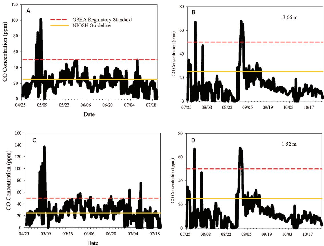
Figure 2. Time series of rolling 8-h average concentrations of carbon monoxide measured in the storage warehouse of the pellet mill. (A) and (B) show the CO measured at 3.66 m above the floor, while (C) and (D) show the measurements at 1.52 m during the two measurement periods.
