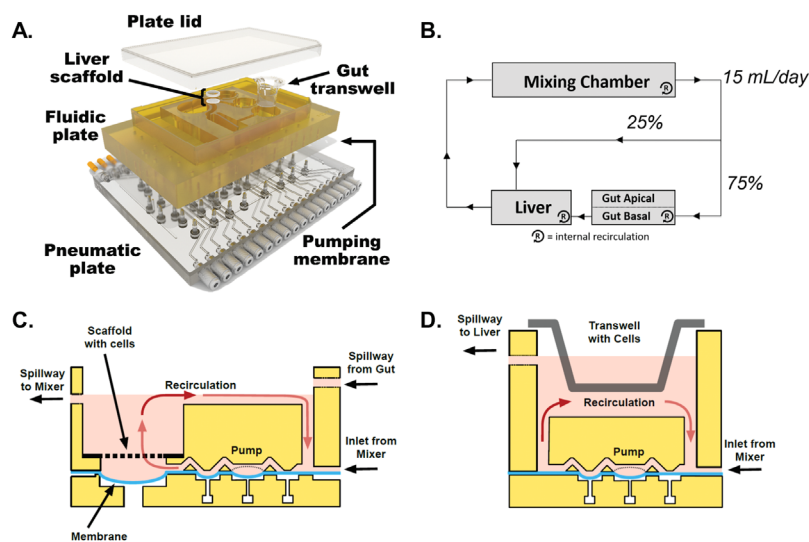
Figure 1. Overview of platform design and operation. (A) Exploded view of a multi-MPS platform. Top plate (shown in yellow polysulfone) contains MPS compartments and distributes culture medium through micromachined channels and pumps on its bottom face. Bottom plate (shown in clear acrylic) distributes compressed air and vacuum to small ports below each pump/valve chamber. A membrane layer (translucent polyurethane) clamped between the two plates seals the channels and provides a sterile barrier while serving as the actuation layer of the pumps and valves. Stainless steel screws fasten the layers together into a single unit that can be handled like a traditional well plate. (B) A flow partitioning schematic illustrates the gut-liver communication circuit and intra-MPS mixing within each compartment. (C) Schematic of the perfused liver MPS on platform (not to scale). The liver module contains a rigid, perfused polystyrene scaffold with 301 microchannels that serve to localize and aggregate primary human hepatocytes and Kupffer cells into miniature liver tissues. A recirculation pump ( 1 \mu\text{L/s} ) maintains continuous flow across a region of shallow geometry to provide efficient oxygenation, while a suspended portion of the pumping membrane serves as a capacitor to smooth the pressure profile of the peristaltic pump. The module integrates fluid inputs from the mixing chamber and gut compartment, while shunting excess volume back to the mixer via an outflow spillway. (D) Schematic of the perfused gut MPS on platform (not to scale). A recirculation pump ( 0.25 \mu\text{L/s} ) maintains continuous flow across basal side of the gut MPS to provide continuous mixing. The module receives fluid input from the mixing chamber while shunting excess volume to the liver compartment via an outflow spillway.
