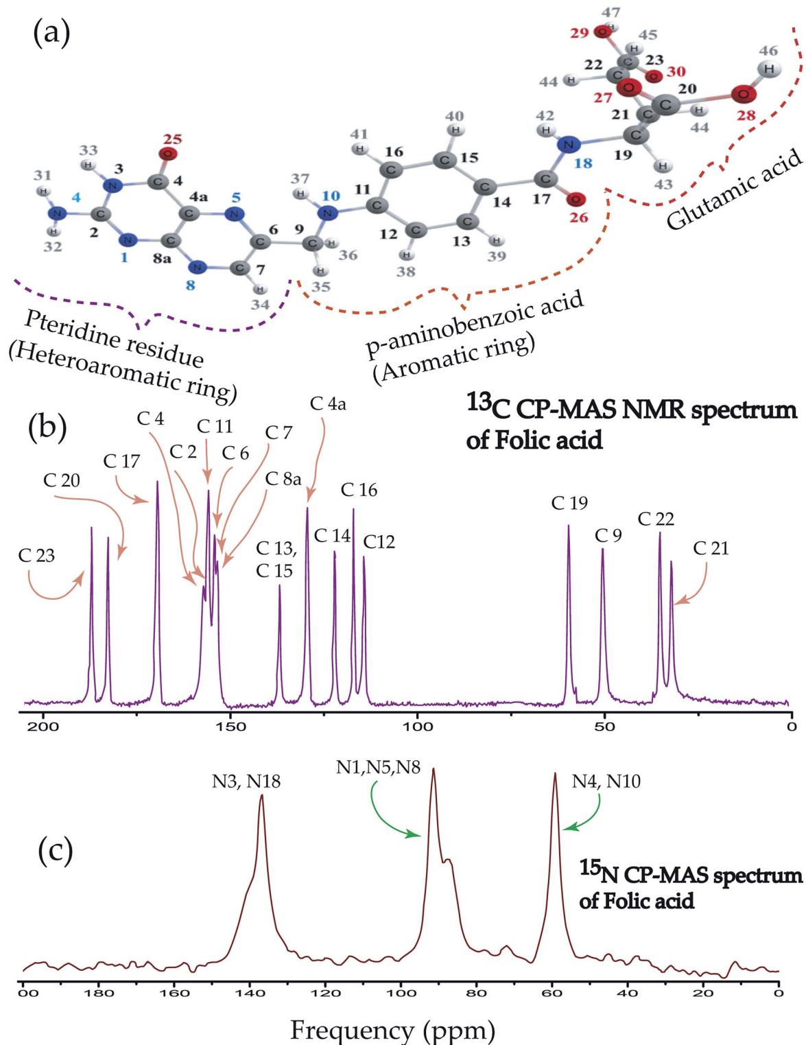
Fig. 1 (a) Folic acid is fabricated by 2 S -2-([4-(2-amino-4-hydroxypteridin-6-yl)-methyl]amino)phenyl formamido pentanedioic acid. It is composed of pteridine, p -aminobenzolate and glutamate moieties. (b) 13 C CP-MAS spectrum of folic acid. (c) 15 N CP-MAS spectrum of folic acid.
