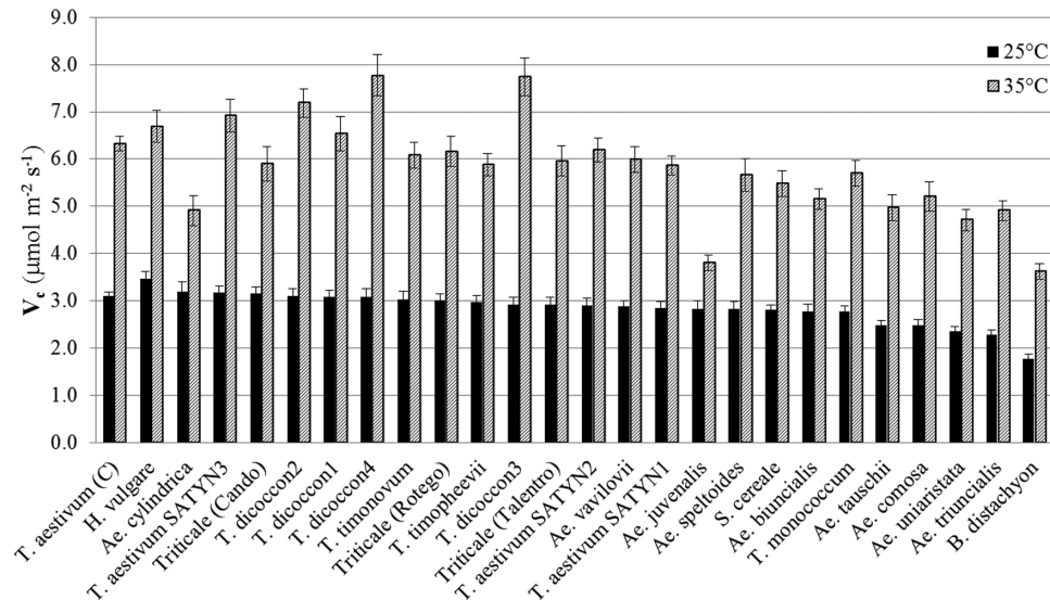
Fig. 1. Rubisco carboxylation velocity ( V_c ) at 25 °C (black bars) and 35 °C (hatched bars) in 25 Triticaceae genotypes. Data organized in decreasing rank at 25 °C, except for T. aestivum cv Cadenza, which is shown on the far left-hand side for comparison.
