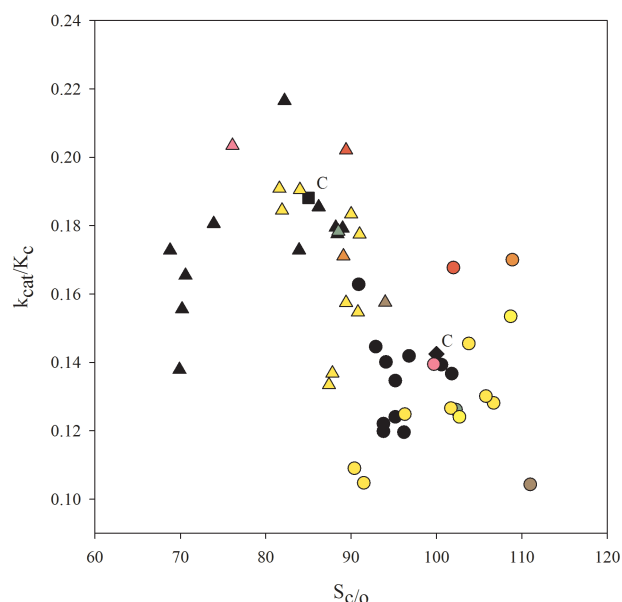
Fig. 4. The relationship between the catalytic efficiency of Rubisco at 21% O_2 ( k_{cat}/K_c , \mu M s^{-1} ) and the specificity factor ( S_{c/o} ) of Rubisco at 25 °C (circles) and 35 °C (triangles). Each colour denotes an rbcL sequence (as per Table 3) and Cadenza wheat (C, used as reference) is represented by the diamond and square at 25 and 35 °C, respectively.
