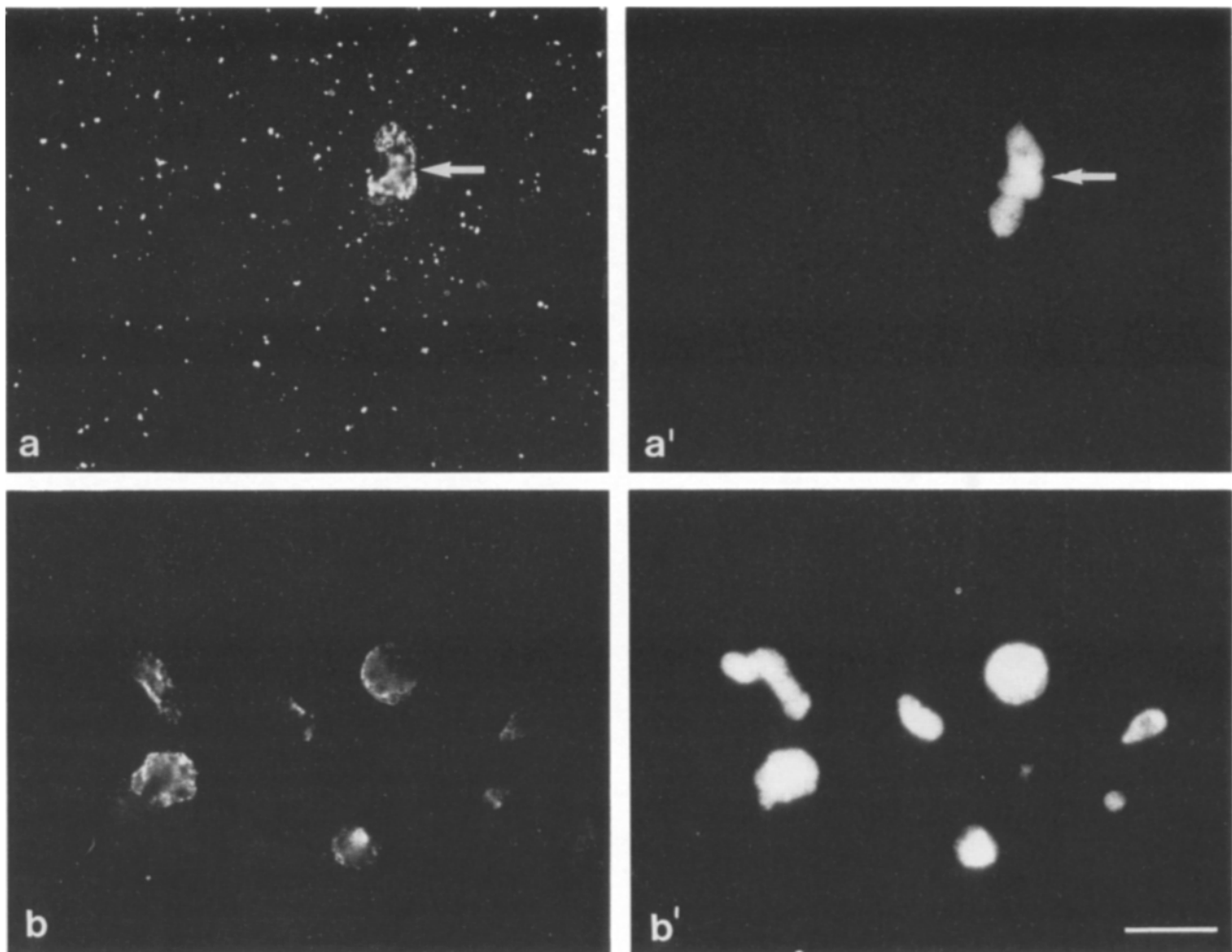
Figure 6. Inhibition of annulate formation by addition of chromatin in form of demembrated Xenopus sperm nuclei. Egg extract was incubated for 2 h in the presence of 600 (a) and 30,000 (b) demembrated sperm nuclei per microliter extract and processed for immunofluorescence microscopy using the pore-specific antibody PII (a and b). The corresponding Hoechst fluorescence is shown in a' and b'. Annulate lamellae form only in presence of low chromatin concentrations as indicated by the numerous fluorescent dots (a). The decondensed sperm chromatin has acquired a nuclear envelope with pore complexes as judged from the rim staining (a, arrow and b). Bar, 20 \mu m.
