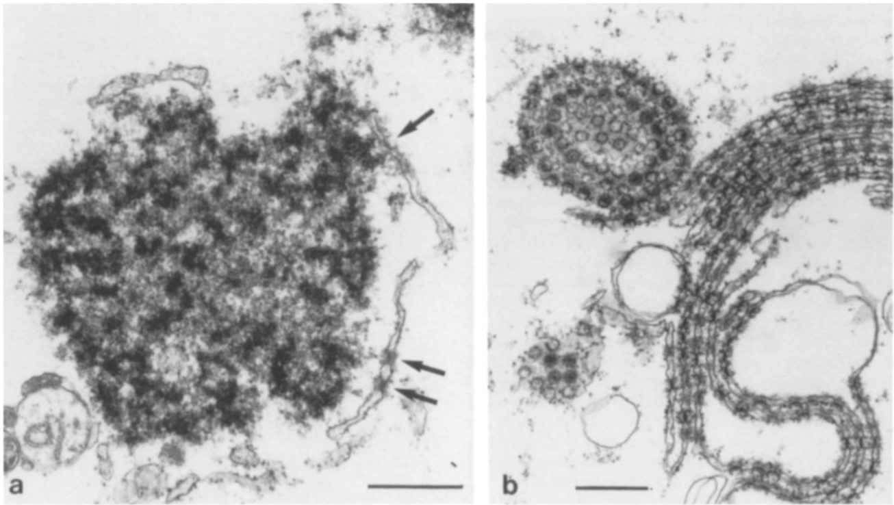
Figure 7. Antilamin antibodies inhibit formation of nuclear envelopes but not of annulate lamellae. Egg extract was incubated with lambda DNA in the presence of antibody S49H2 for 2 h and then prepared for EM. Only a few nuclear envelope fragments, some with pore complexes ( arrows ), are associated with the chromatin surface ( a ). In contrast, stacks of annulate lamellae have formed normally ( b ). Bars, 0.5 \mu\text{m} .
