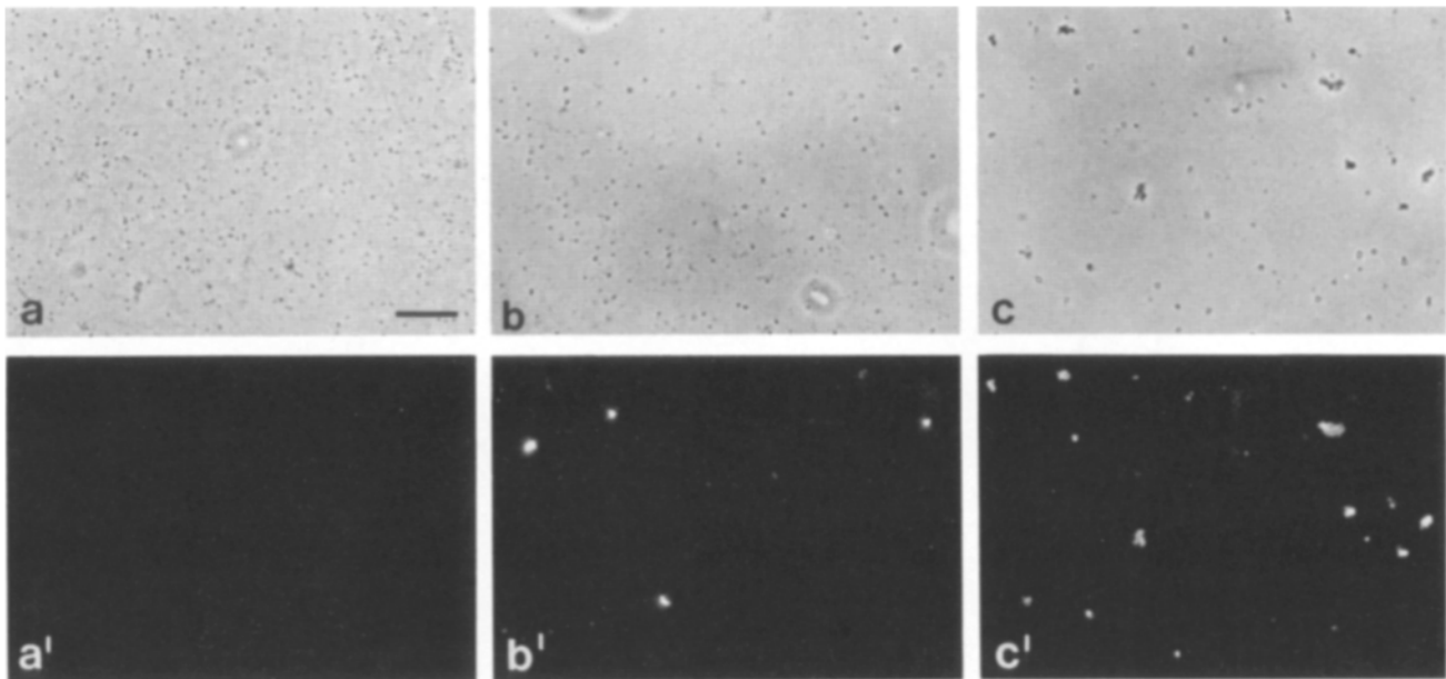
Figure 4. Time course of annulate lamellae formation in egg extract incubated without DNA as revealed by immunofluorescence microscopy using the pore-specific antibody P11 ( a' , 0 min; b' , 30 min; c' , 60-min incubation). The corresponding phase-contrast images are shown in a-c . Bar, 20 \mu m.
