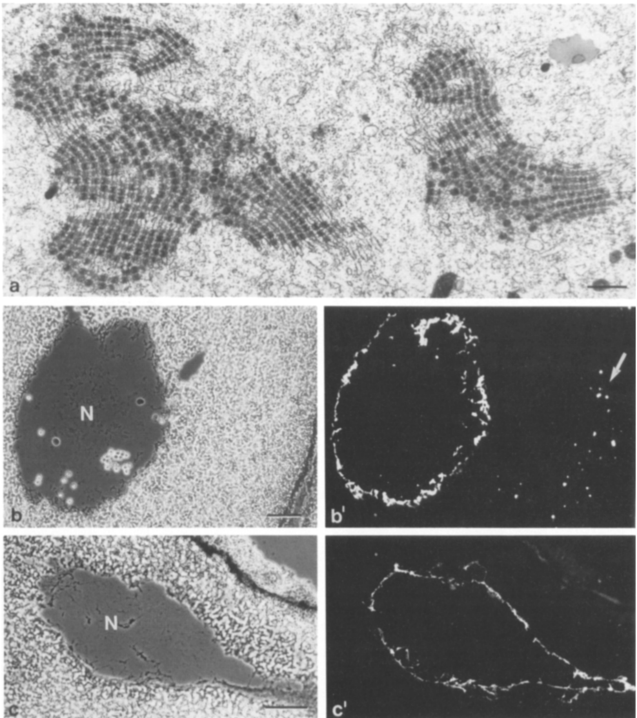
Figure 1. Annulate lamellae in Xenopus laevis oocytes. The electron micrograph of an ultrathin section ( a ) shows stacks of annulate lamellae in the ooplasm. Note the high pore density. Immunofluorescence microscopy using the pore-specific antibody PII reveals the distribution of annulate lamellae in a cryosectioned Xenopus oocyte ( b' ). Antibody PII stains the nuclear envelope ( N , nucleus) as well as numerous annulate lamellae that are located preferentially in the periphery of the oocyte ( arrow in b' ; shown here is a full-grown oocyte). In contrast, antilamin antibody S49H2 stains exclusively the nuclear periphery ( c' ). The corresponding phase-contrast images are shown in b and c . Bars: ( a ) 0.5 \mu\text{m} ; ( b and c ) 50 \mu\text{m} .
