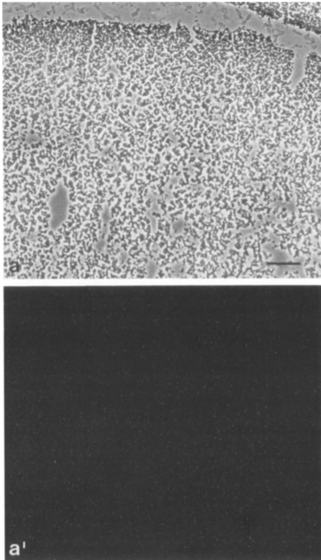
Figure 2. Absence of annulate lamellae in Xenopus eggs. A frozen section was incubated with antibody P11 followed by Texas red-labeled secondary antibodies and viewed with epifluorescence ( a' ) and phase-contrast ( a ) optics. Bar, 50 \mu\text{m} .
