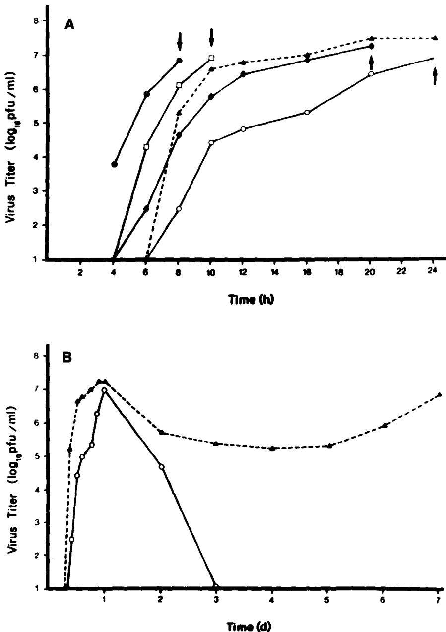
FIG. 1. Virus production from L (solid lines) and LM-K (dashed lines) cells inoculated at various m.o.i.'s. Cultures of L cells were inoculated at m.o.i.'s of 10 (●), 1 (□), 0.1 (◆), and 0.01 (○). LM-K cells were inoculated at an m.o.i. of 10 (▲). Panel (A) short-term (1 day); Panel (B) long-term (7 days). Arrows refer to times of complete fusion of the monolayers.
