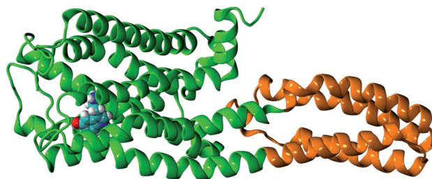
Fig. 1 The structure of the G-protein coupled 5-HT 1B receptor (green) bound to serotonin (in VDW representation) along with mini-G 0 (orange).
