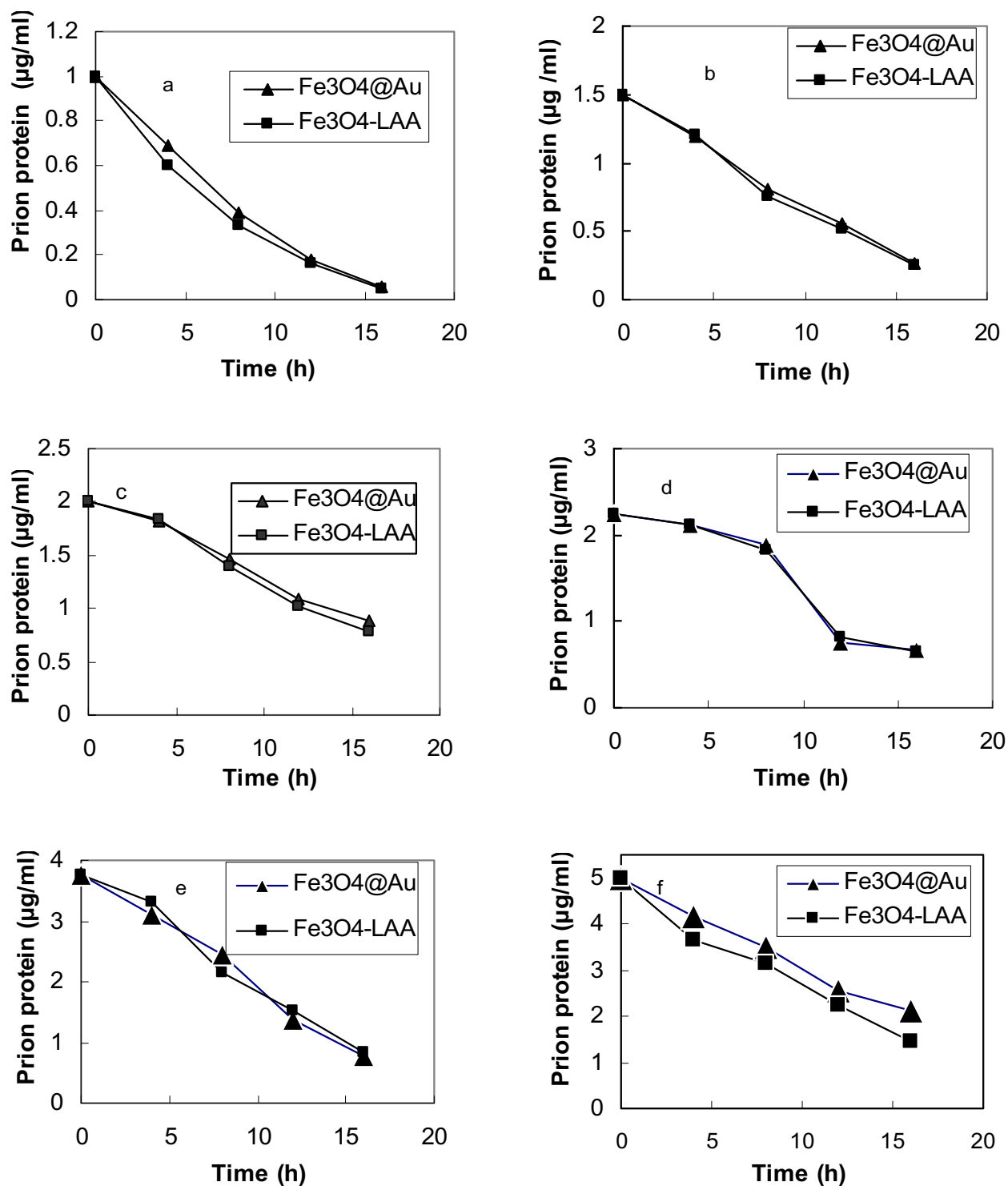
Figure 6 Plots of huPrPrec binding onto \text{Fe}_3\text{O}_4\text{@Au} and \text{Fe}_3\text{O}_4\text{-LAA} (a) as a function of time for various concentrations of huPrPrec.
