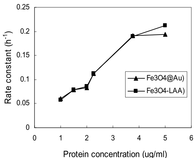
Figure 7 Dependence of the rate constants of huPrPrec binding on the concentrations of reacting huPrPrec.
