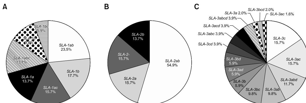
Fig. 3. Percentile share of swine leukocyte antigen ( SLA ) class I-based groups within the investigated herd. Clustering based on SLA-1 (A), SLA-2 (B), and SLA-3 (C) profiles. Within the investigated herd there were 7 of 8 identifiable combinations of the SLA-1 profile, four (all possible) versions of SLA-2 genes, and 14 of 16 possible combinations of SLA-3 . The most often repetitive SLA-1 profile was SLA-1ab , found in 23.5% of the analyzed specimens. More than half of the herd (54.9%) demonstrated a homologous SLA-2 genes profile: SLA-2ab and SLA-3c profiles, together with SLA-3ac , the most abundantly occurring profile among the herd (15.7% each).
