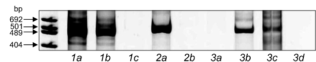
Fig. 2. A representative swine leukocyte antigen ( SLA ) class I pattern of an analyzed porcine blood sample. This specimen represents the SLA class I profile, SLA-1ab 2a 3bc (polymerase chain reaction products: 548, 548, 585, 565, and 533 bp, respectively).
