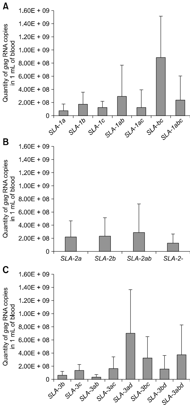
Fig. 4. Average porcine endogenous retrovirus (PERV) viremia within SLA-1 (A), SLA-2 (B), and SLA-3 (C) profile-based groups. Statistically significant differences in PERV gag RNA level were observed only in the SLA-1 profile-based group (A). SLA-1bc group displayed significantly higher viremia than that in the SLA-1a , 1b , 1c , and 1ac profiles. No correlation with PERV viremia and the SLA-2 (B) or SLA-3 profiles (C) was detected. SLA , swine leukocyte antigen.
