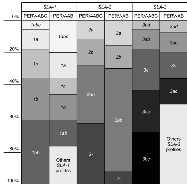
Fig. 6. Distribution of particular swine leukocyte antigen ( SLA ) class I profiles within the assessed herd. Classes were divided into two subgroups: with and without porcine endogenous retrovirus (PERV)-C subtype in their genome (left and right column, respectively, for each hue). In the PERV-C-positive group, the highest occurrences were in the following SLA class I profiles: SLA-1 , ab; SLA-2 , ab; and SLA-3 , c. The SLA-1ab and SLA-3c profiles were present almost twice as often in the PERV-C-positive specimens than in the PERV-C-negative specimens.
