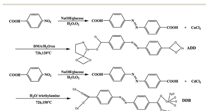
Scheme 1 Synthetic routes to ADD and DDB .
