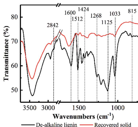
Fig. 6 FT-IR spectrum of the de-alkaline before/after PHP pretreatment.
