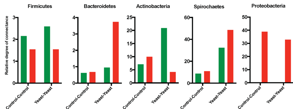
Figure 6. The impact of yeast supplementation on the relative degree of connectance of main bacterial phyla. Co-occurrence Network inference (CoNet) was used to measure the relative degree of connectance of main bacterial phyla within (a) cecum and (b) colon microbiota of yeast supplemented (Yeast-Yeast) and control (Control-Control) piglets. Grouped bar charts show the total number of significant positive (co-occurrence; color code green) or negative (mutual exclusion; color code red) relationships of bacterial genera belonging to main phyla divided by the mean relative abundance of each phylum.
