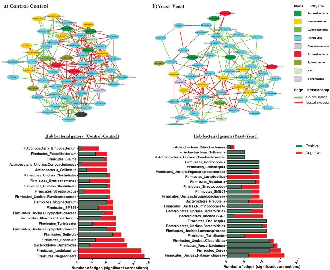
Figure 4. Influence of yeast supplementation on the structure and co-occurrence pattern of the microbiota of cecum contents. Co-occurrence Network inference (CoNet) was used to explore interrelationships of bacterial genera within the microbiota of cecum contents of (a) control and (b) pre-and post-weaning yeast supplemented piglets (Yeast-Yeast). Network constructs on the top panel depict the interrelationships of nodes (i.e. bacterial genera, colored based on originating phylum) using positive (co-occurrence; green) or negative (mutual co-exclusion; red) edges. Each edge represents a significant relationship (FDR q < 0.05 ) supported by at least three out of four measures of similarity/correlation (including Pearson's, Spearman's, Bray-Curtis, and Kullback-Leibler). Stacked bar charts show the distribution of hub bacterial genera (i.e. those showing the highest number of significant positive or negative relationships) within the microbiota of each treatment group. Color codes have been used to depict the number of positive (green) and/or negative (red) relationships of hub genera. *Due to the high relative importance of actinobacterial genera in shaping the structure of the community, these genera have been included in bar charts irrespective of their total number of relationships.
