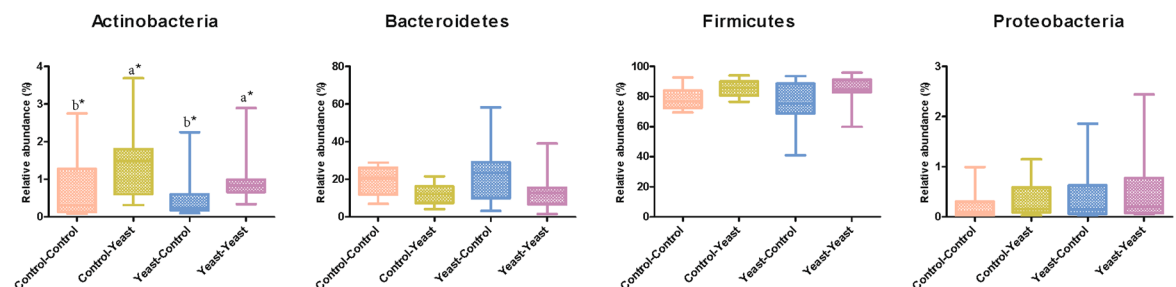
Figure 3. Effect of yeast-supplementation on the proportion of main bacterial phyla of piglets' hindgut microbiota. Box-Whiskers plots show the proportion of main bacterial phyla (above 1% of the community) in the microbiota of (a) cecum and (b) colon contents of piglets collected on day 28 post-weaning. The X-axis shows pre- and post-weaning yeast supplementation regimens including Control-Control, Control-Yeast, Yeast-Control, and Yeast-Yeast. Boxes. Boxes denote interquartile range, with a line at the median, while whiskers show minimal and maximal observations in the data set. Superscripts denote significant differences ( P < 0.05 ) between the means. * P -values have been calculated based on log-transformed proportions.
