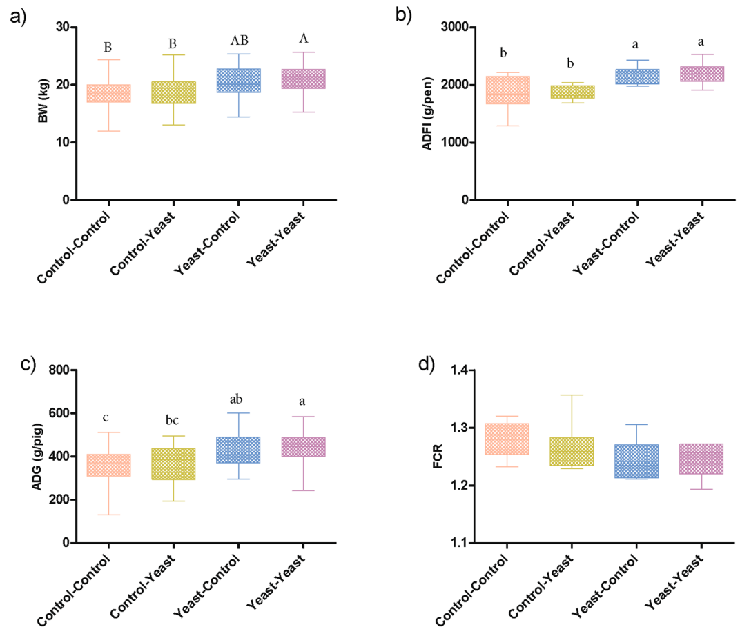
Figure 1. Effect of yeast-supplementation on zootechnical performance parameters of piglets. Box-Whisker plots have been used to compare zootechnical performance parameters of piglets among different pre- and post-weaning yeast supplementation regimens including Control-Control, Control-Yeast, Yeast-Control, and Yeast-Yeast. Parameters compared included: (a) final day (day 28 post-weaning) body weight, (b) average daily feed intake (g per pen of four piglets), (c) average daily weight gain (g per piglet), and (d) feed conversion ratio calculated per pen of four piglets. Boxes denote interquartile range, with a line at the median, while whiskers are indicating minimal and maximal observations for each parameter. Superscripts denote significant difference ( P < 0.05 ; a–c) or statistical trend ( P < 0.1 ; A, B).
