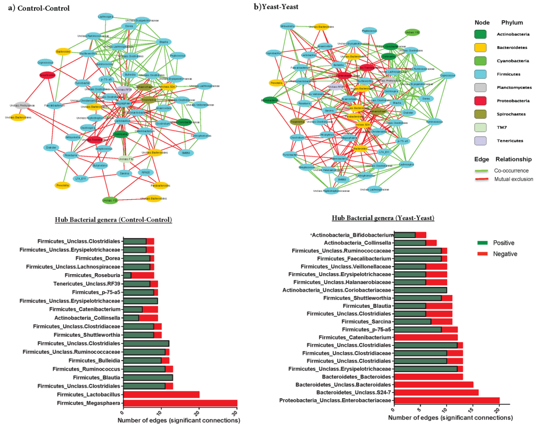
Figure 5. Influence of yeast supplementation on the structure and co-occurrence pattern of the microbiota of colon contents. Co-occurrence Network inference (CoNet) was used to explore interrelationships of bacterial genera within the microbiota of colon contents of (a) control and (b) pre- and post-weaning yeast supplemented piglets (Yeast-Yeast). Network constructs on the top panel depict the interrelationships of nodes (i.e. bacterial genera, colored based on originating phylum) using positive (co-occurrence; green) or negative (mutual exclusion; red) edges. Each edge represents a significant relationship (FDR q < 0.05 ) supported by at least three out of four measures of similarity/correlation (including Pearson's, Spearman's, Bray-Curtis, and Kullback-Leibler). Stacked bar charts show the distribution of hub bacterial genera (i.e. those showing the highest number of significant positive or negative relationships) within the microbiota of each treatment group. Color codes have been used to depict the number of positive (green) and/or negative (red) relationships of hub genera. *Due to the high relative importance of actinobacterial genera in shaping the structure of the community, these genera have been included in bar charts irrespective of their total number of relationships.
