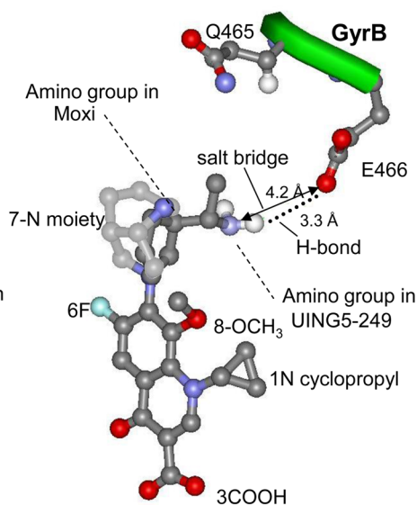
Figure 5. Location of C-7 ring substituents relative to amino acid 466 of GyrB in cleaved complexes. A potential salt bridge and hydrogen bond between the C-7 ring systems and GyrB-466E are shown. (A) Dione binding. The C-7 ring system of UING5-157 is shown in light gray, whereas that of UING5-207 is in dark gray. (B) Quinolone binding. The C-7 ring system of moxifloxacin is shown in light gray, whereas that of UING5-249 is in dark gray.
