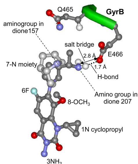
Figure 5. Location of C-7 ring substituents relative to amino acid 466 of GyrB in cleaved complexes. A potential salt bridge and hydrogen bond between the C-7 ring systems and GyrB-466E are shown. (A) Dione binding. The C-7 ring system of UING5-157 is shown in light gray, whereas that of UING5-207 is in dark gray. (B) Quinolone binding. The C-7 ring system of moxifloxacin is shown in light gray, whereas that of UING5-249 is in dark gray.
