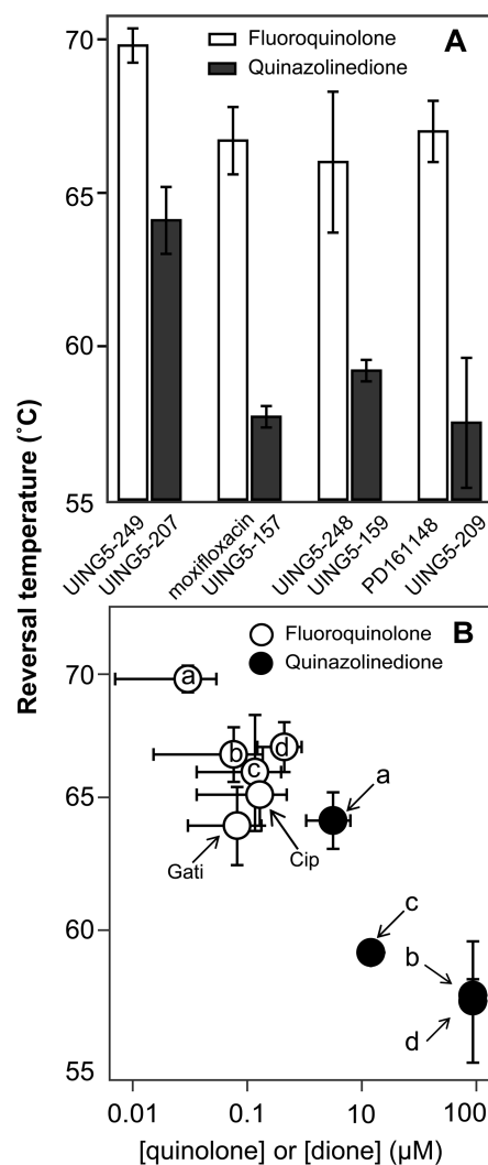
Figure 3. Thermal reversal of cleaved complexes formed with quinolones and diones. (A) Comparison of quinolones and cognate diones. Cleaved complexes were formed as described in Methods and then incubated at various temperatures to determine the temperature causing 50% resealing of DNA. (B) Relationship between drug concentration required for complex formation and thermal resealing of DNA. Concentrations of fluoroquinolone (empty circles) or quinazolinodione (filled circles) required to trap 20% of the plasmid DNA in a linear form were determined as in Figure 1B, and temperatures at which 50% of the linear DNA was resealed were determined. Letters indicate paired fluoroquinolones and diones (a = UING5-249/207; b = moxifloxacin/UING5-157; c = UING5-248/159; d = PD161148/UING5-209); Cip, ciprofloxacin; Gati, gatifloxacin. Error bars indicate standard deviation of the mean.
