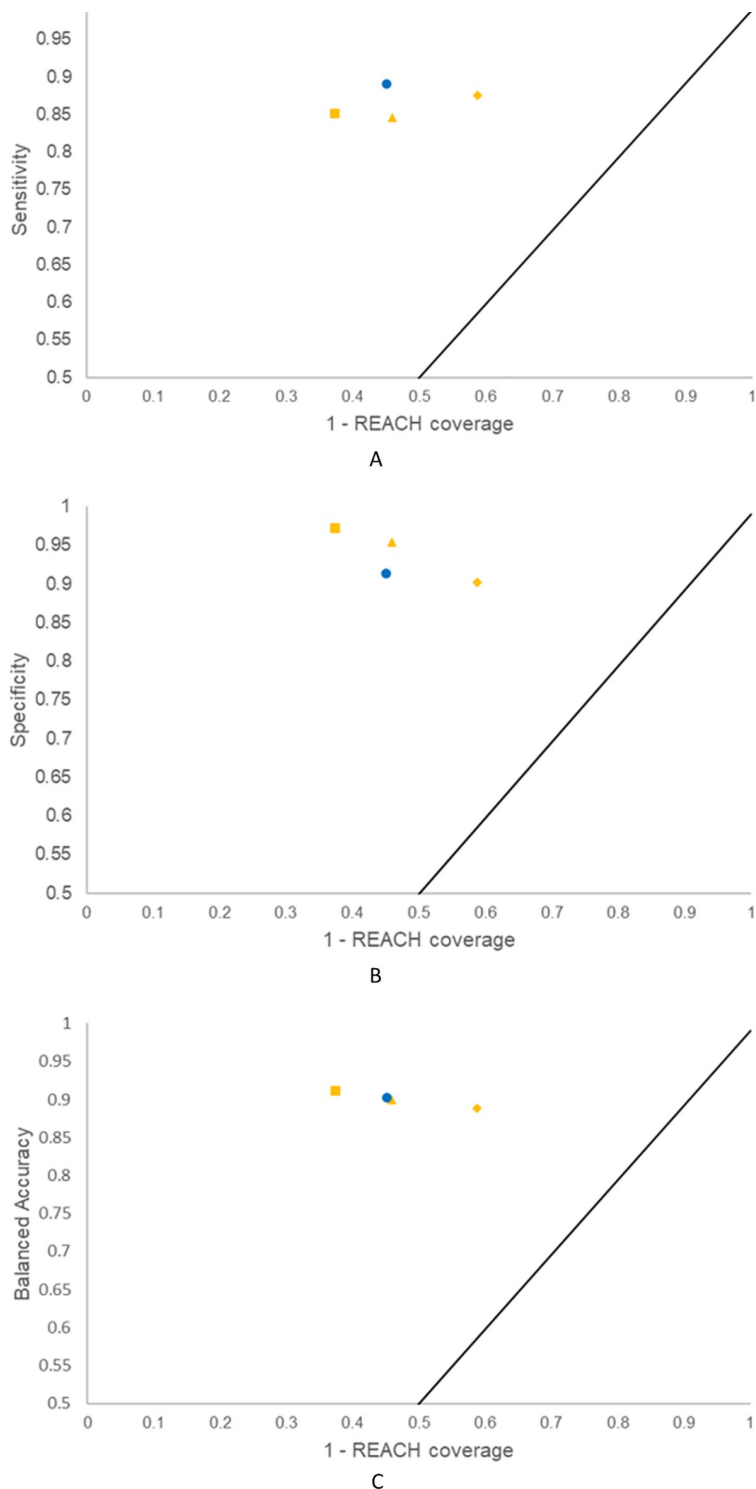
Fig 4. Performance of QSAR2:1, QSAR3:1, QSAR4:1 and QSAR4:1R vs. REACH coverage. The performance is described by Sensitivity (A), Specificity (B) and Balanced Accuracy (C). The following tokens correspond to the rational selection approach: a yellow diamond for QSAR2:1, a yellow triangle for QSAR3:1 and a yellow square for QSAR4:1. The blue circle corresponds to the random selection approach for QSAR4:1-R.
