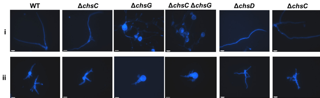
FIG 4 AfCHS is required for the compensatory increase in chitin content in response to caspofungin treatment. CFW-stained fluorescent images of the wild-type (WT) strain and \Delta Afchs mutants in RPMI 1640 alone (i) or supplemented with 2 \mu\text{g/ml} caspofungin (ii) after 12 h at 37°C. Scale bars = 10 \mu\text{m} .
