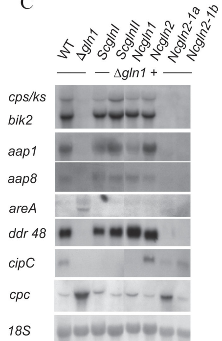
Figure 3. Characterization of heterologous \Delta gln1 complementation mutants. A. Plate assays comparing the growth of the wild type (WT), the \Delta gln1 mutant and different complemented transformants. Complete medium (CM) contained 18 mM glutamine, while the minimal medium (CD) contained no additional nitrogen source. Pictures were taken after 3 days of cultivation. B. Pictures of the wild type (WT), the \Delta gln1 mutant and the heterologous GS complementants grown for 3 days in ICI submerge cultures with either 6 mM glutamine (gln) (GA- and bikaverin-inducing (red coloration) conditions) or 60 mM glutamine as nitrogen source. C. Total RNA was isolated from mycelia grown for 5 days in ICI submerge cultures with 6 mM glutamine and used for northern blot analysis. 18S rRNA was visualized as a loading control. Abbreviations: aap1 and aap8 , amino acid transporter genes; cipC , ddr48 and the cross-pathway control gene cpc were found to be GS-target genes [47]; mepB , ammonium transporter gene.
