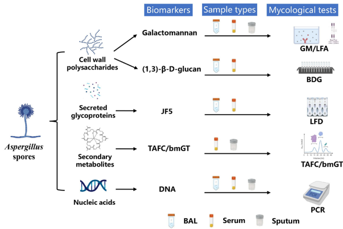
Figure 2 Mycological tests using different sample types for the diagnosis of invasive pulmonary aspergillosis. BAL, bronchoalveolar lavage fluid; GM, galactomannan; BDG, (1,3)- \beta -D-glucan; LFA, lateral flow assay; LFD, lateral flow device; TAFC/bmGT, triacetylfusarinine C or bis(methylthio)gliotoxin.
