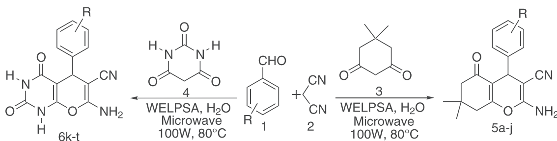
SCHEME 1 Strategic depiction to synthesize tetrahydrobenzo[ b ]pyrans 5a–j and pyrano[2,3- d ]pyrimidinones 6k–t
